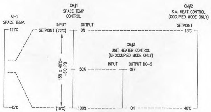
SERVICE BAY DC-9100 SEQUENCE GRAPH COPYRIGHT JOHNSON CONTROLS, INC. 1980
