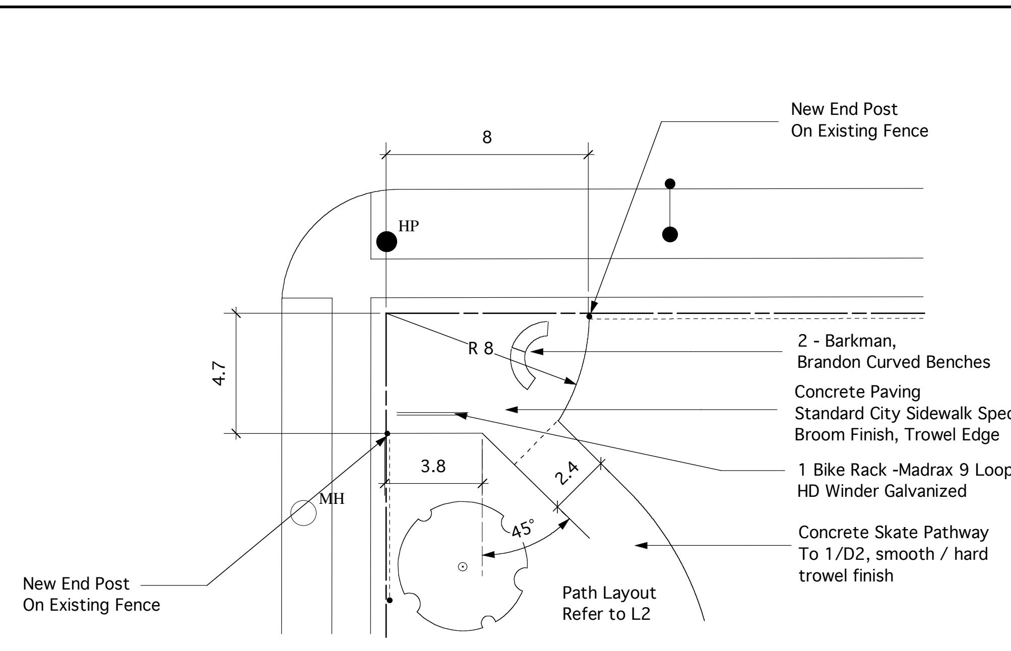
2 NORTH ENTRANCE COURT L4 Scale: 1:150
