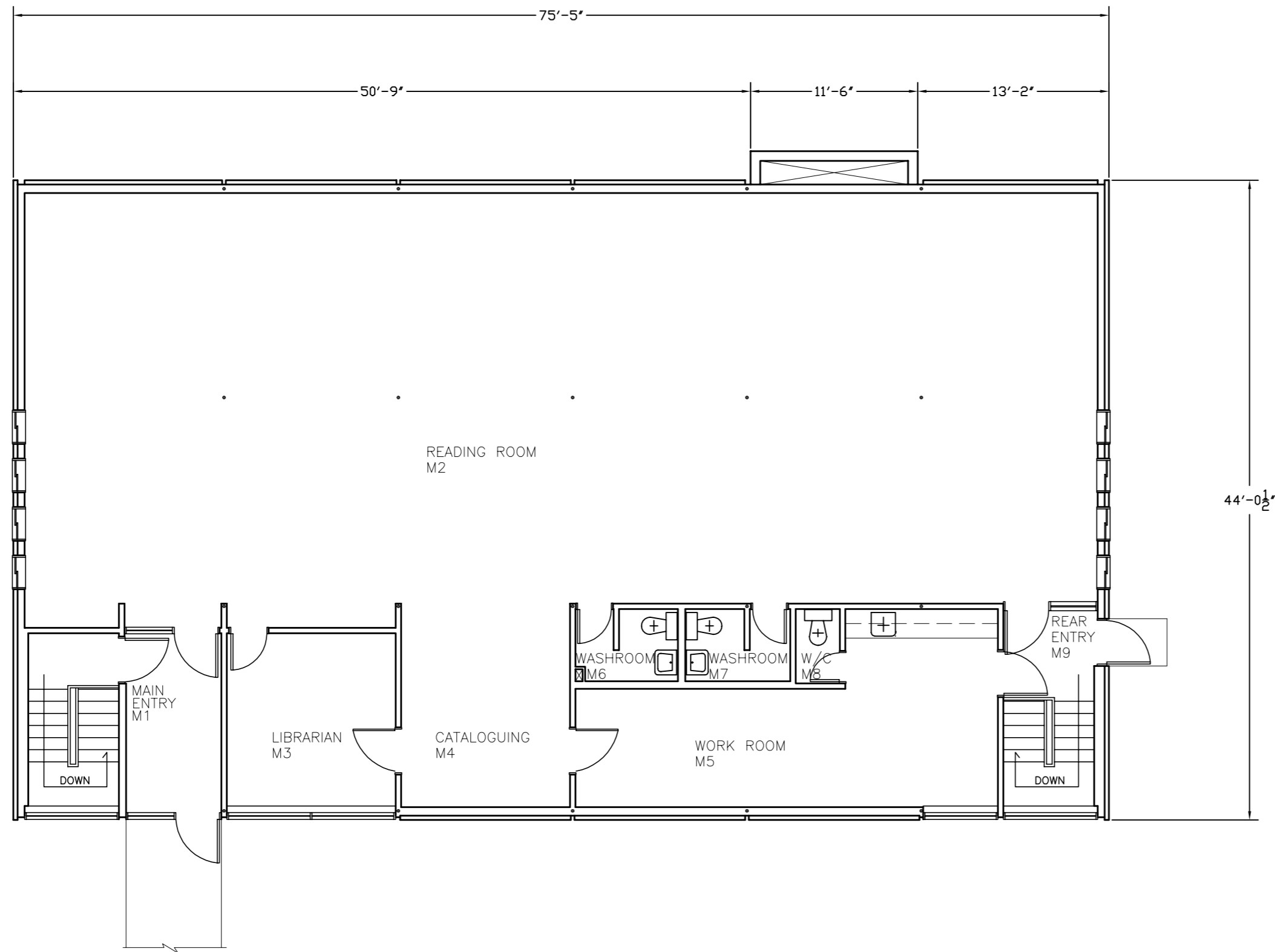
MAIN FLOOR PLAN
