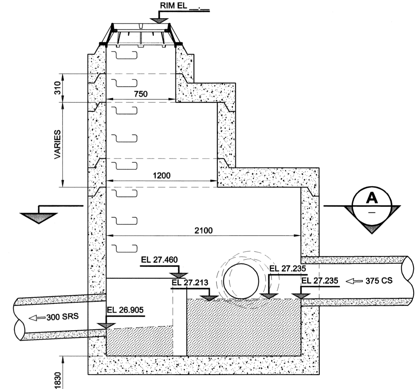
MANHOLE 23 OVERFLOW DETAIL
