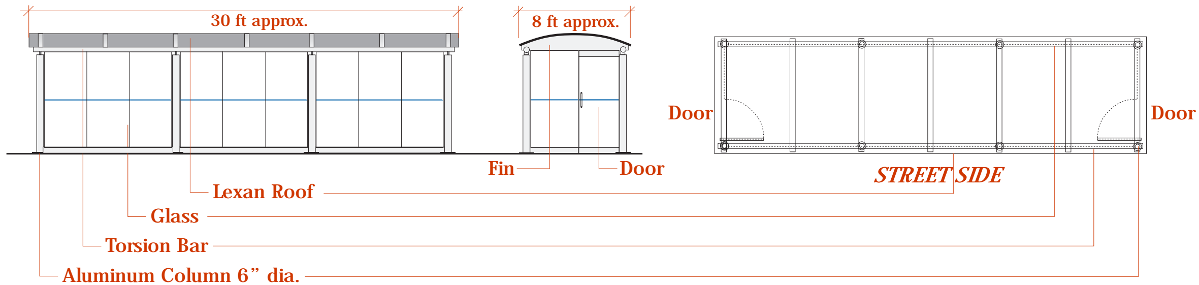
Elevation View
