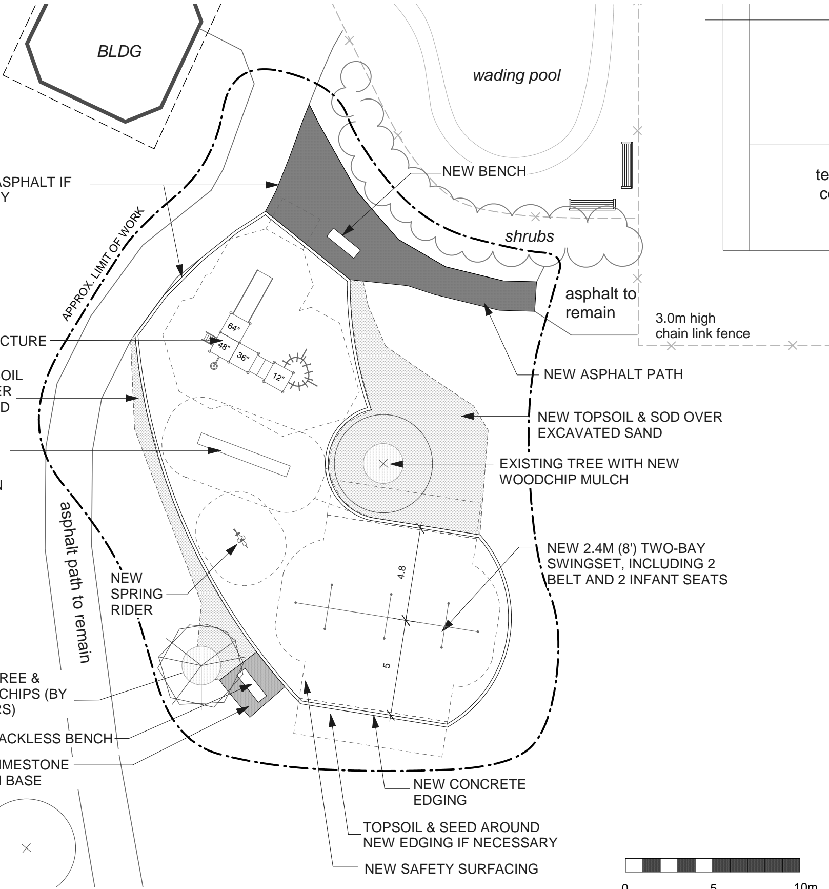
LAYOUT DRAWING (1:300)
