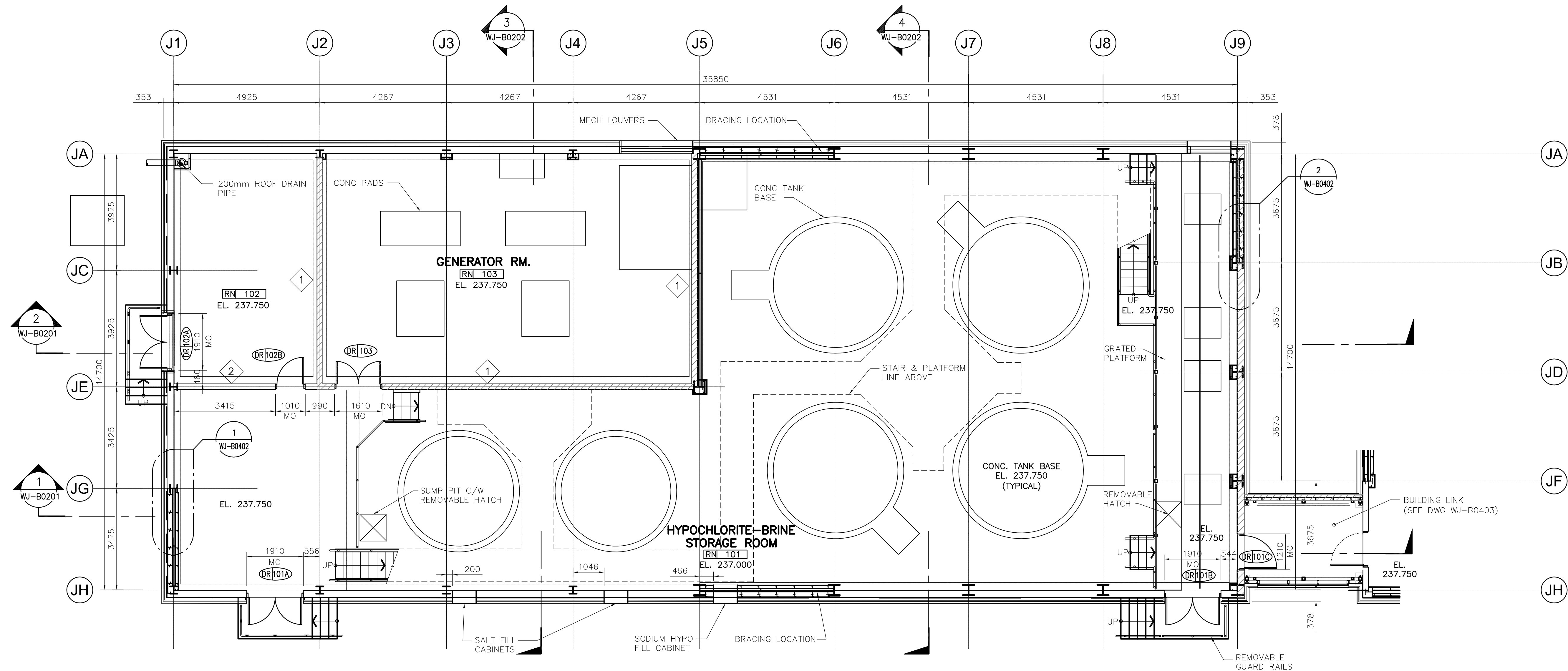
1 MAIN FLOOR PLAN WJ-B0110 1:75
