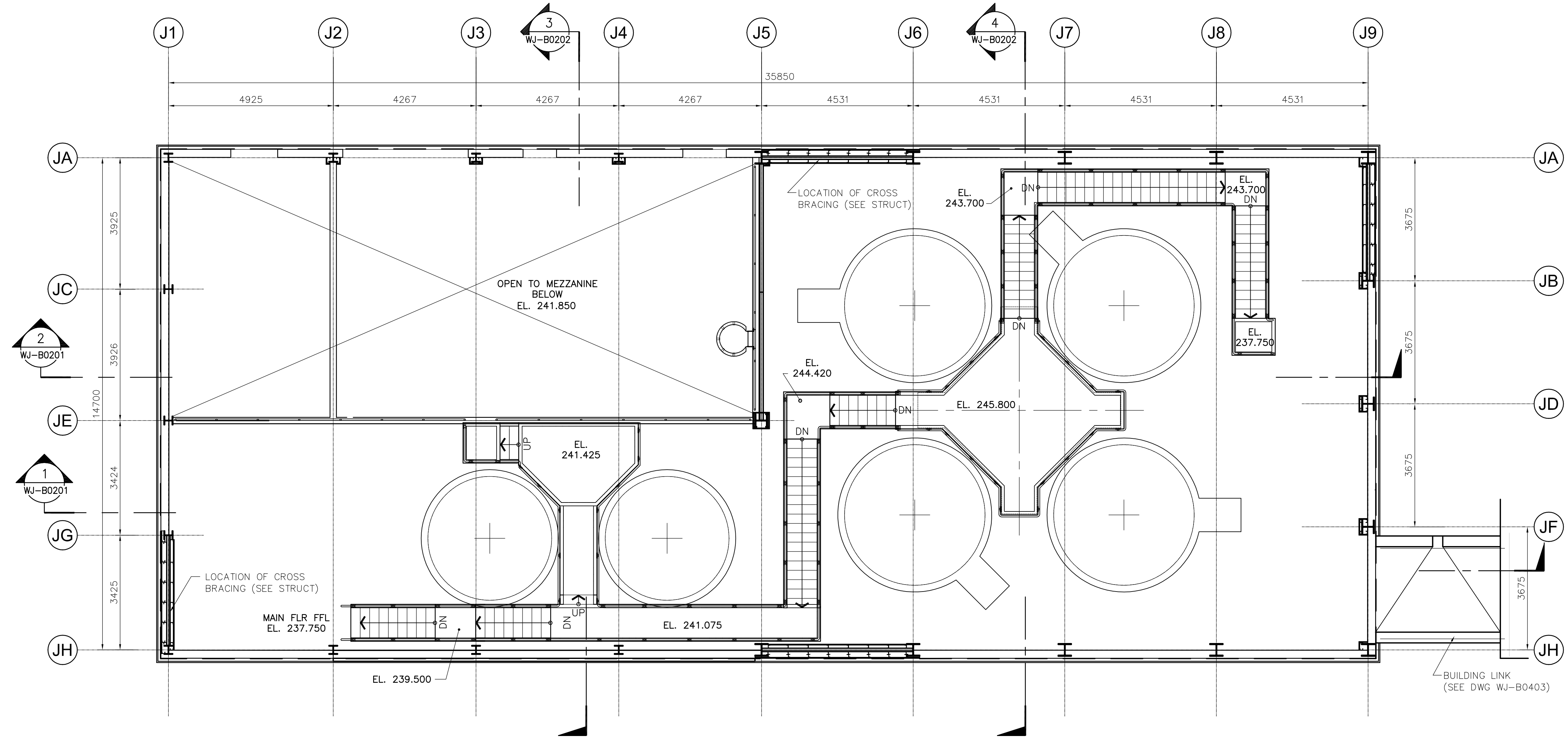
1 CATWALK PLAN WJ-B0120 1:75
