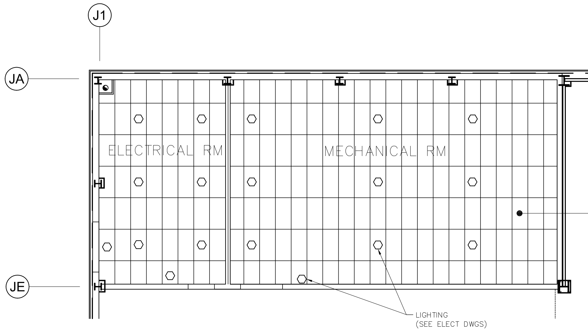
1 ELECT & MECH RM REFLECTED CEILING PLAN WJ-B0121 1:75
