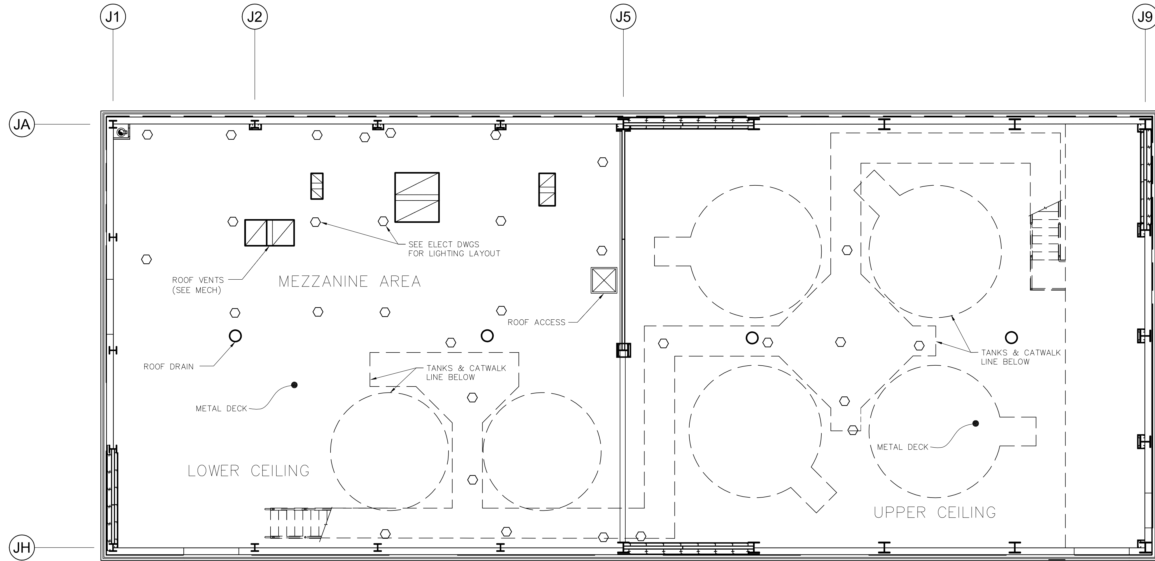
2 MAIN FLOOR REFLECTED CEILING PLAN WJ-B0121 1:75
