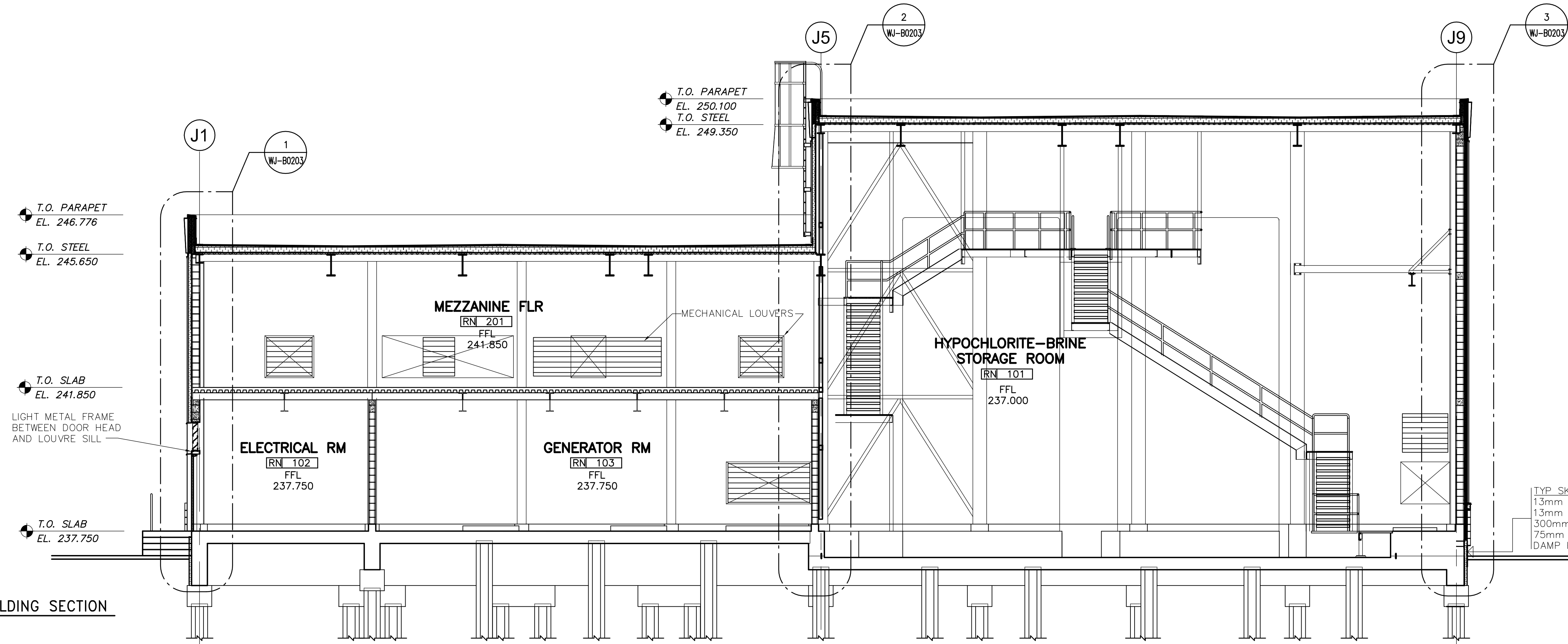
1 BUILDING SECTION WJ-B0110 1:75
