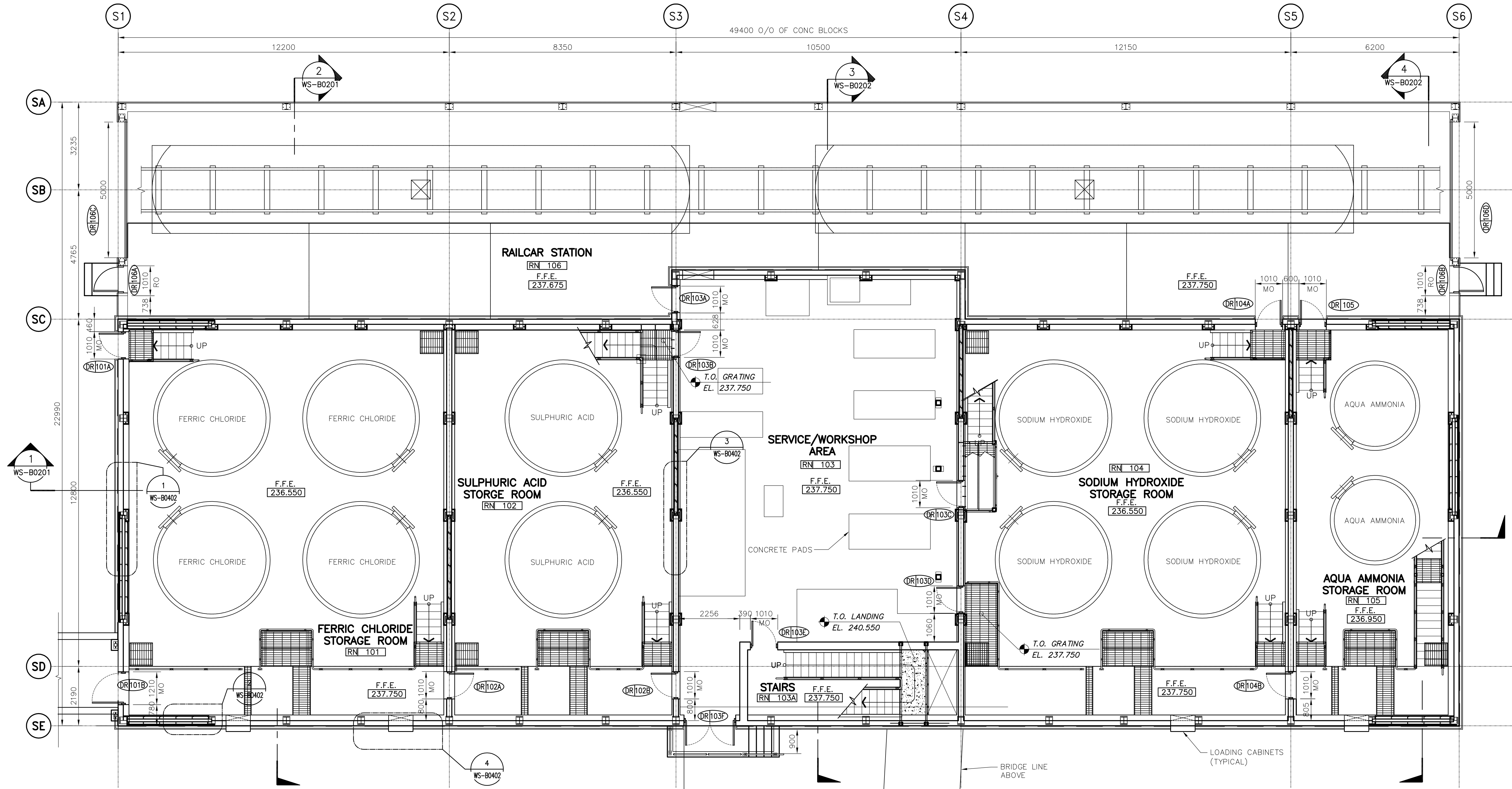
1 MAIN FLOOR PLAN WS-B0110 1:75
