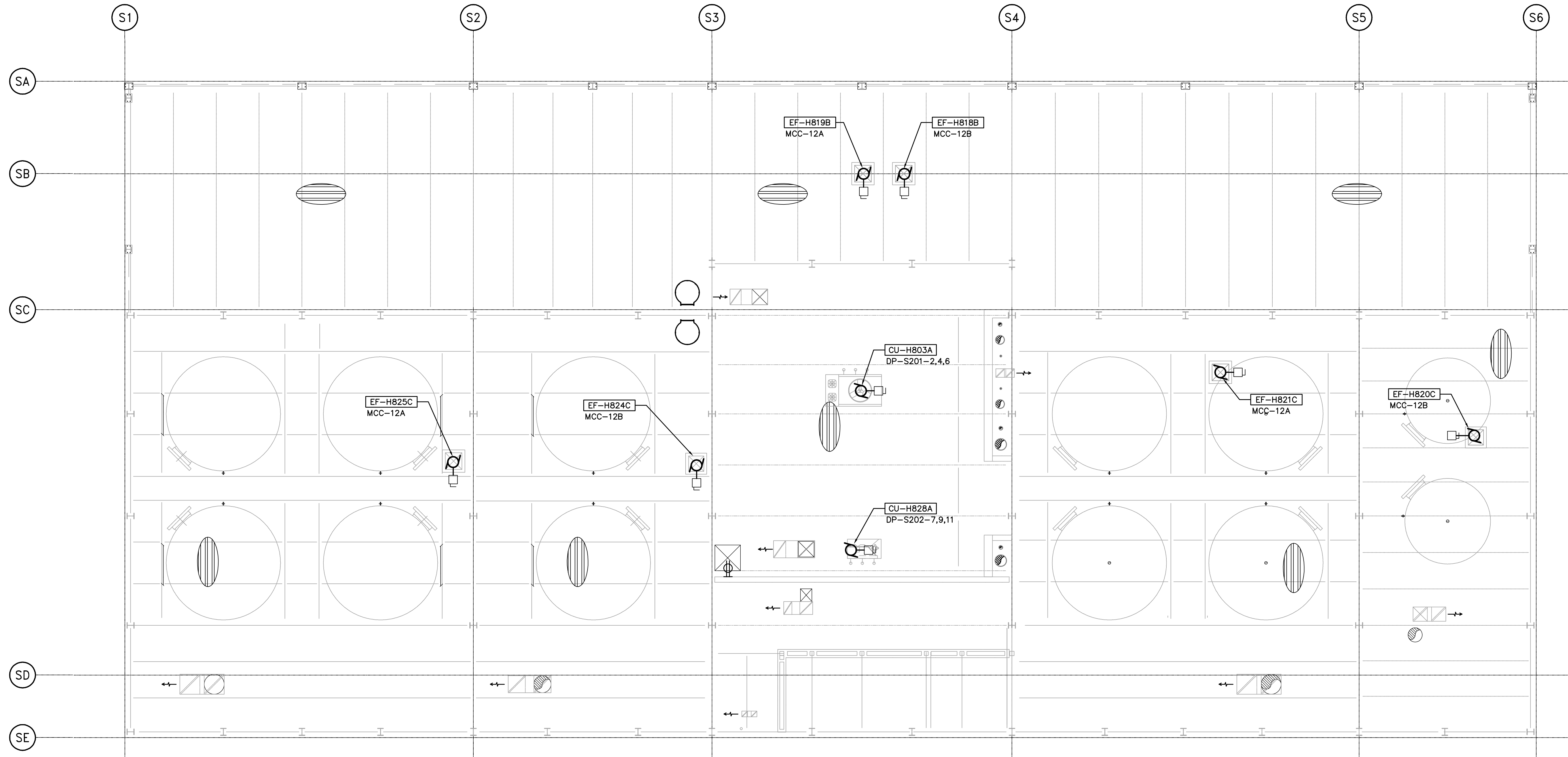
ROOF POWER PLAN 1:75
