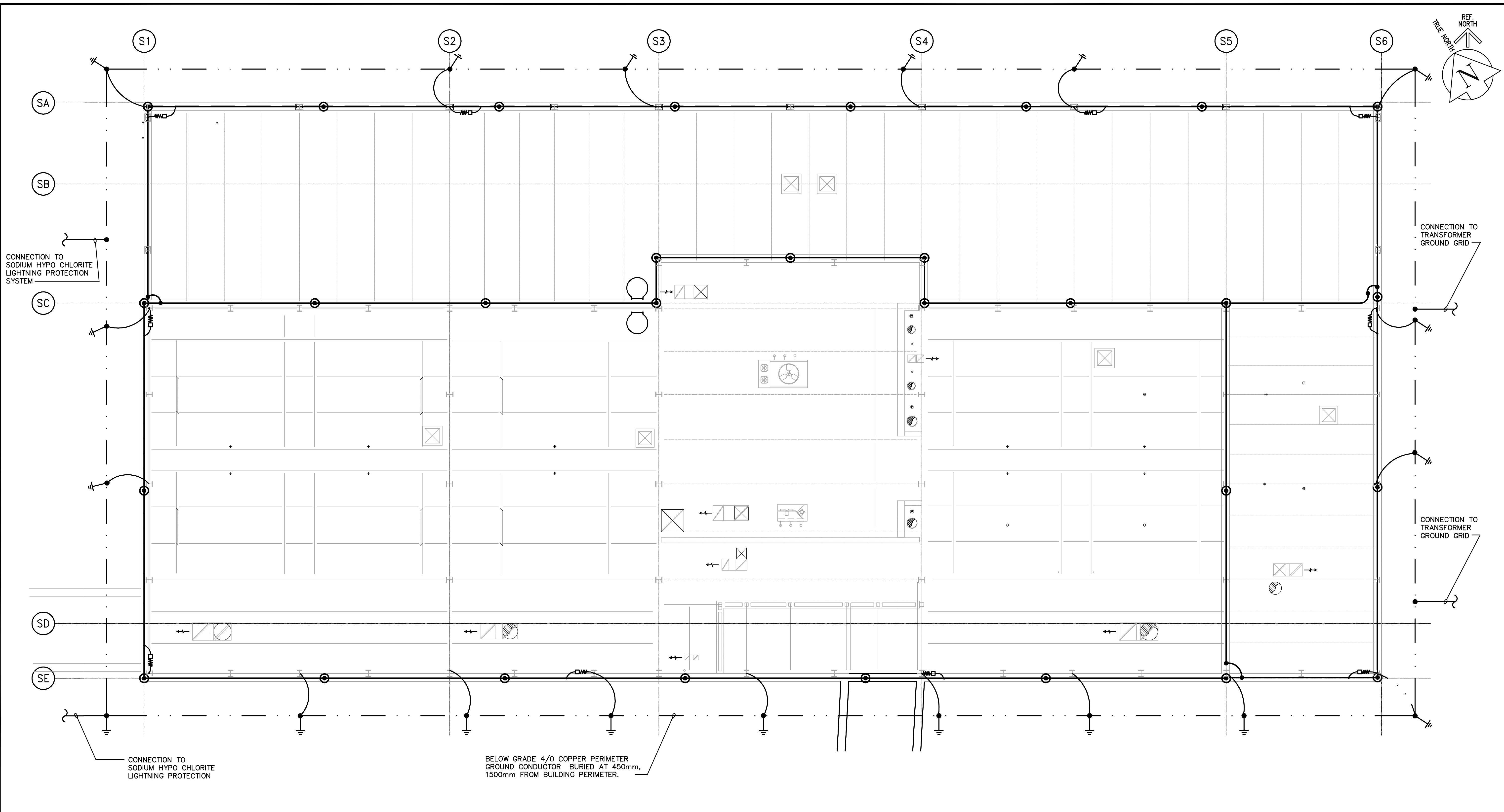
ROOF PLAN 1:75
