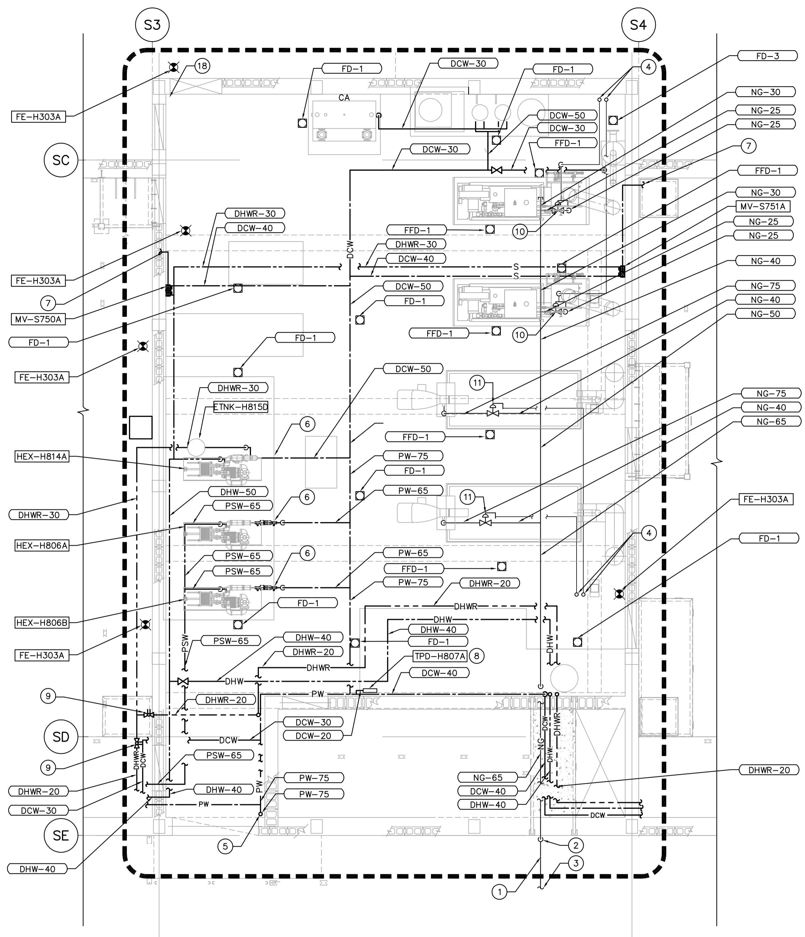
1 PARTIAL MECHANICAL ROOM PLUMBING PLAN 1:50
