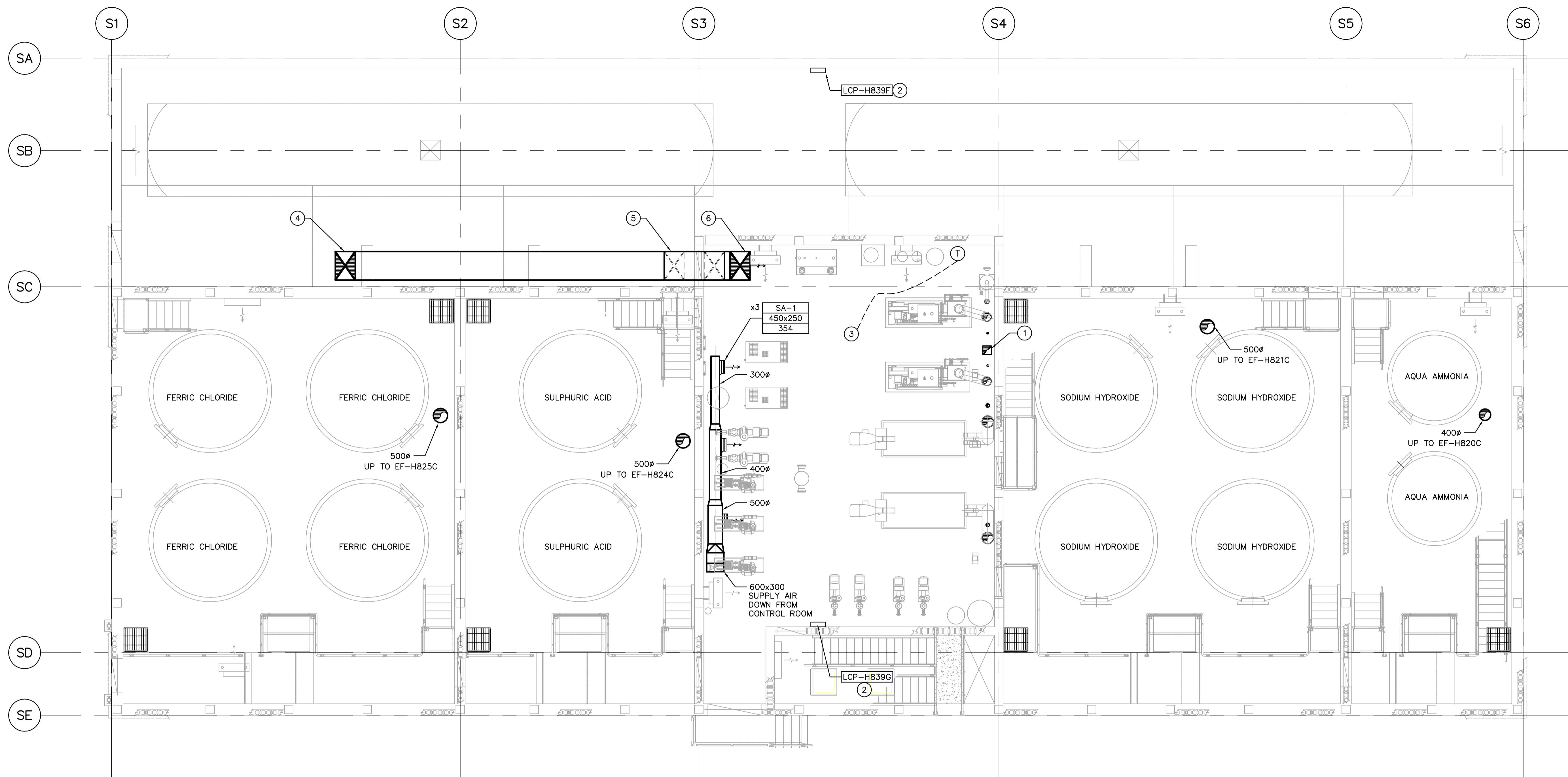
1 MAIN LEVEL VENTILATION PLAN 1:75
