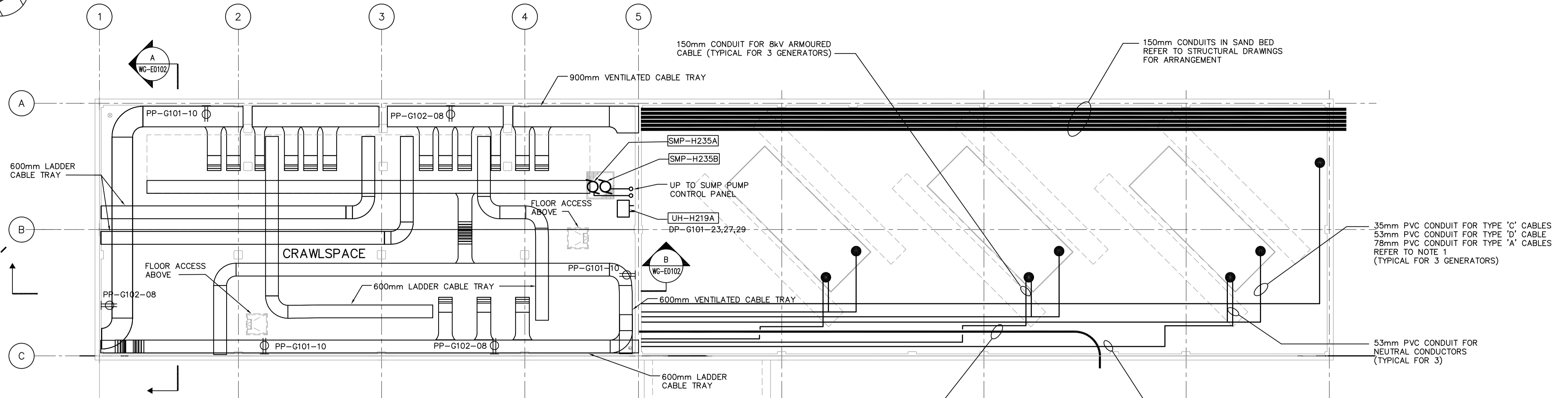
CRAWLSPACE FLOOR PLAN 1:100
