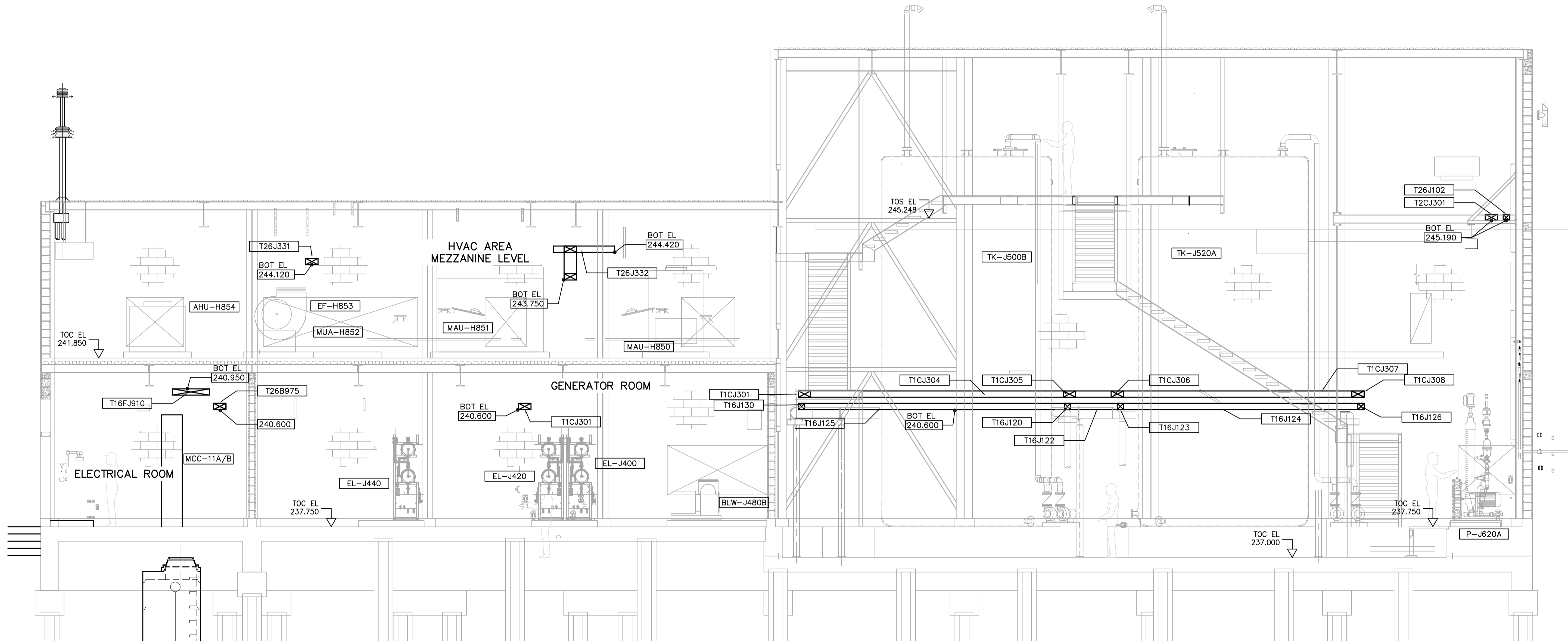
A SECTION WJ-E0111 1:50 WJ-E0121 WJ-E0131
