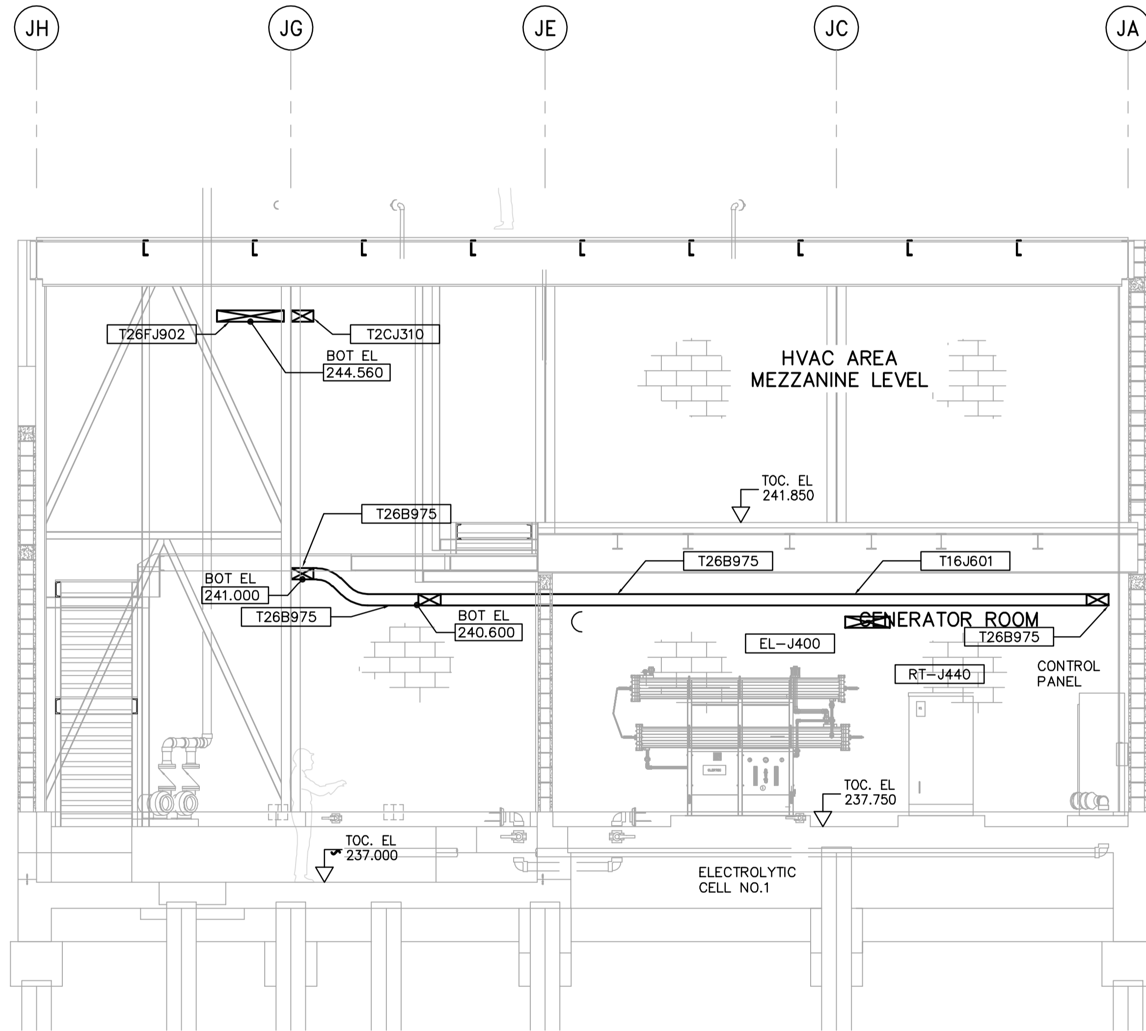
C SECTION WJ-E0111 1:50 WJ-E0121
