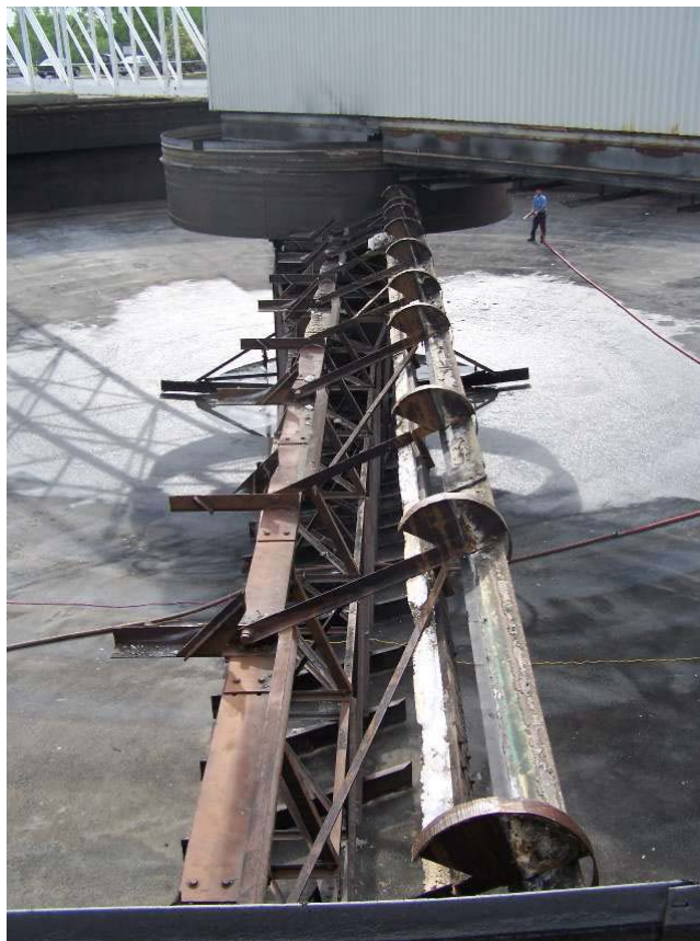
Photo 3-12 Clarifier Drained
