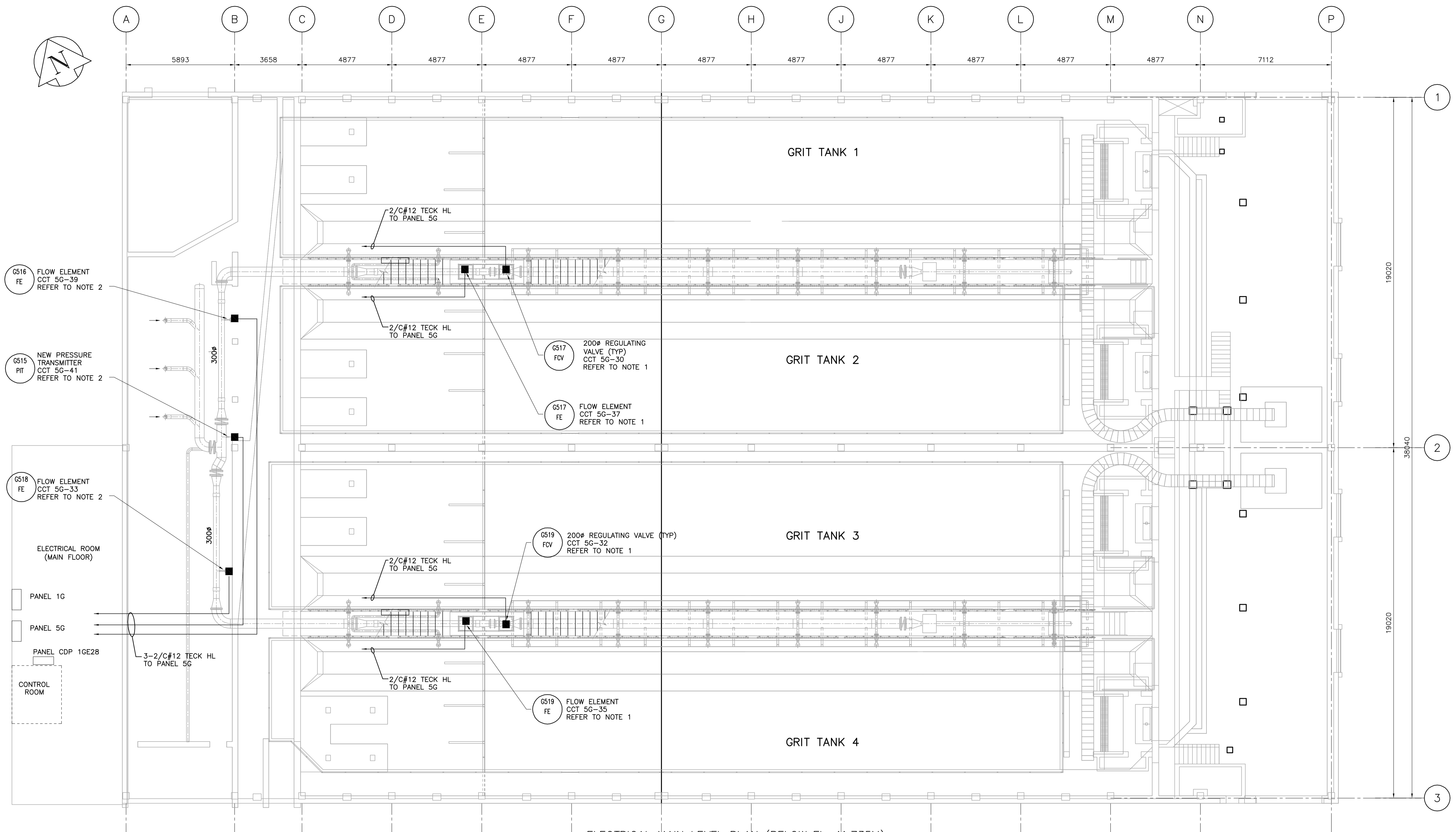
ELECTRICAL MAIN LEVEL PLAN (BELOW EL. 11.735M) SCALE 1:100
