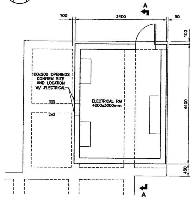
1 PLAN - ELECTRICAL RM 1c SCALE: 1:40
