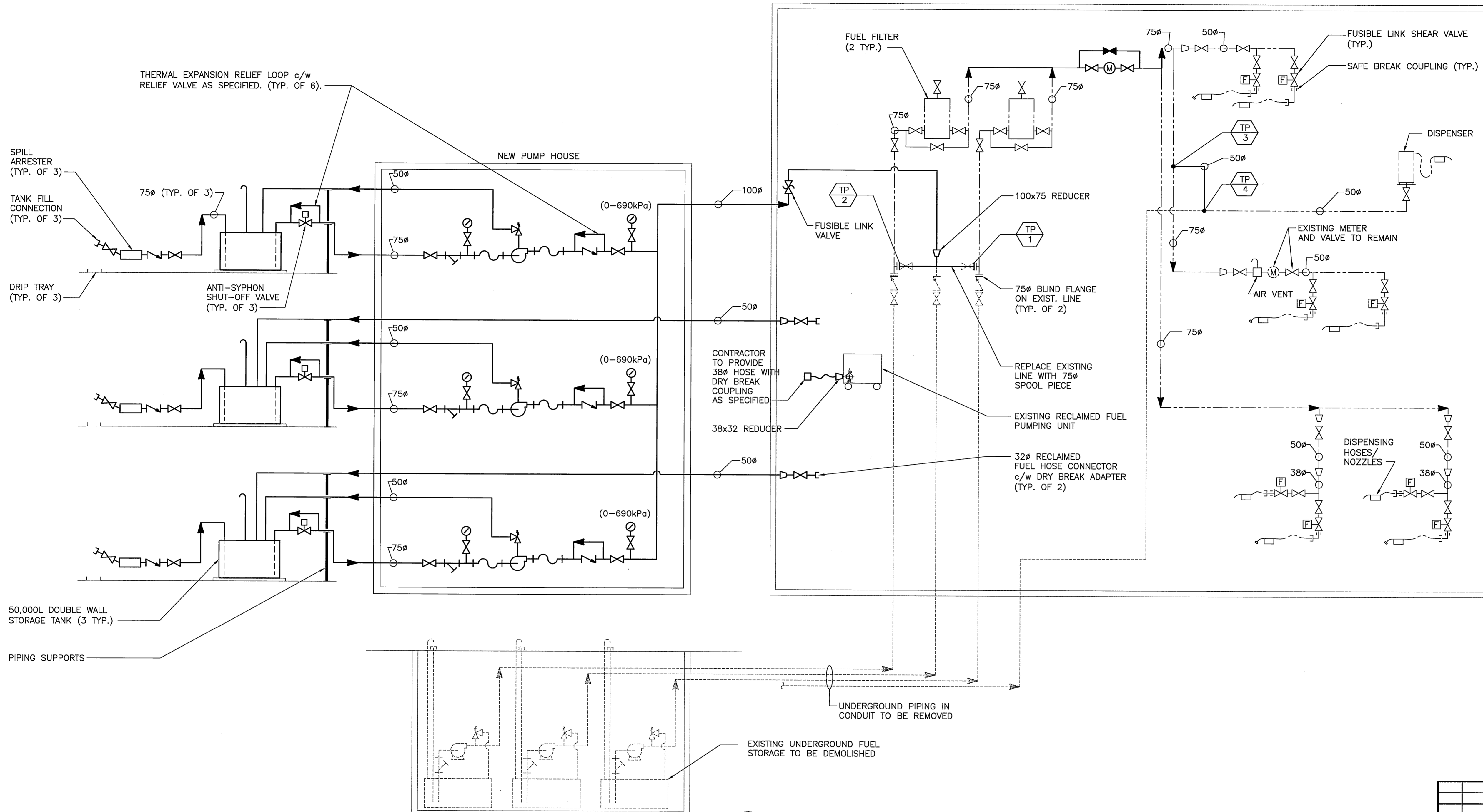
1 DIESEL FUEL SYSTEM N.T.S.
