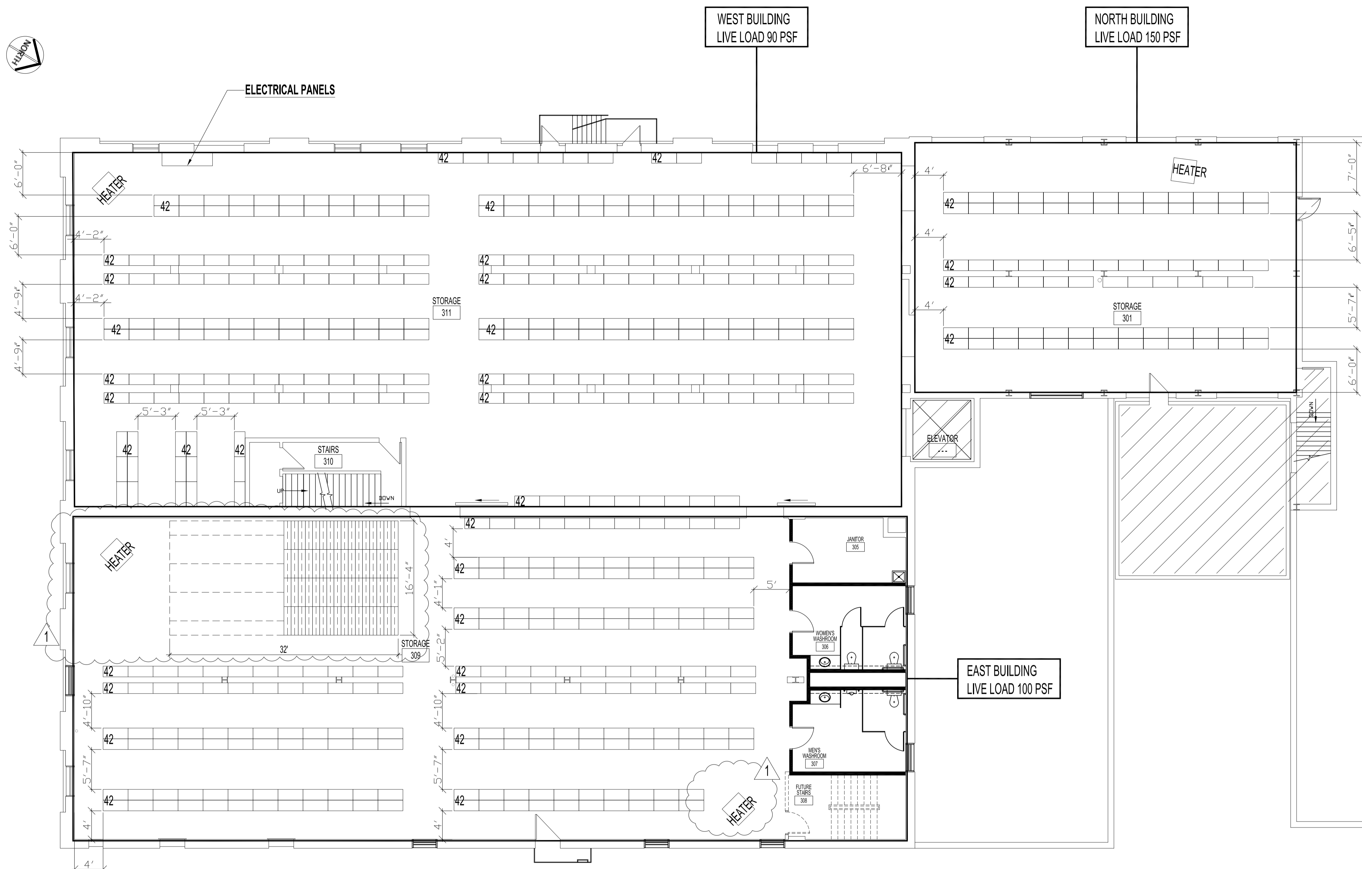
THIRD FLOOR PLAN - SHELVING LAYOUT SCALE: 1/8"=1'-0"
