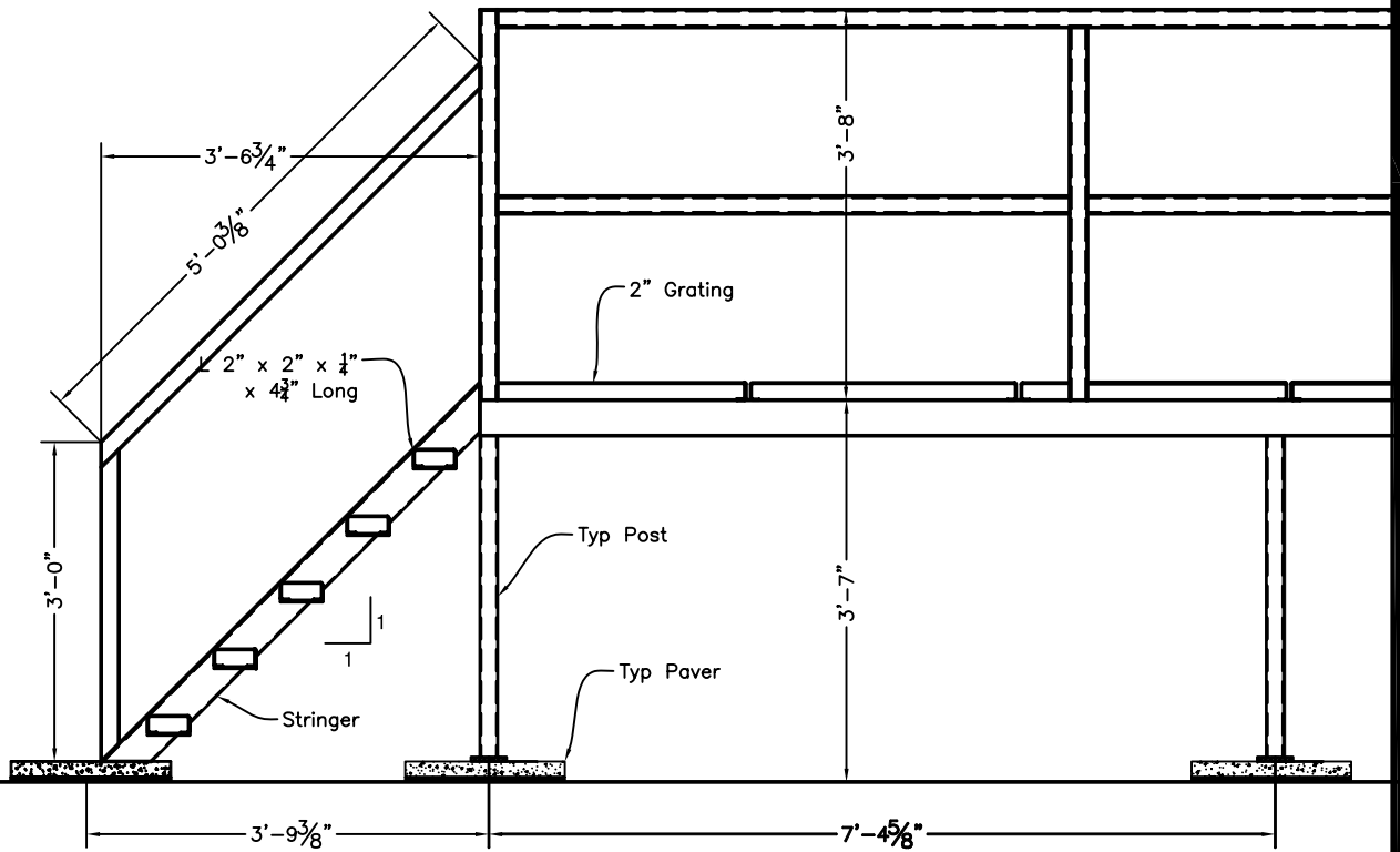
Typical Stair Detail Scale: 1/2" = 1'-0"
