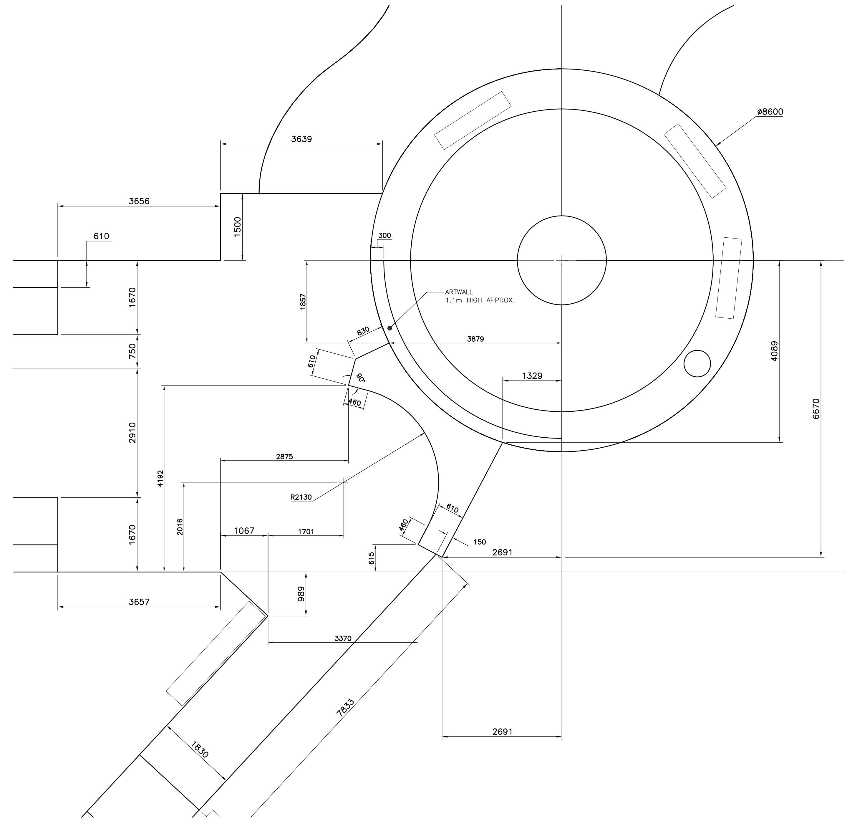
ENTRY PLAZA DIMENSIONS
