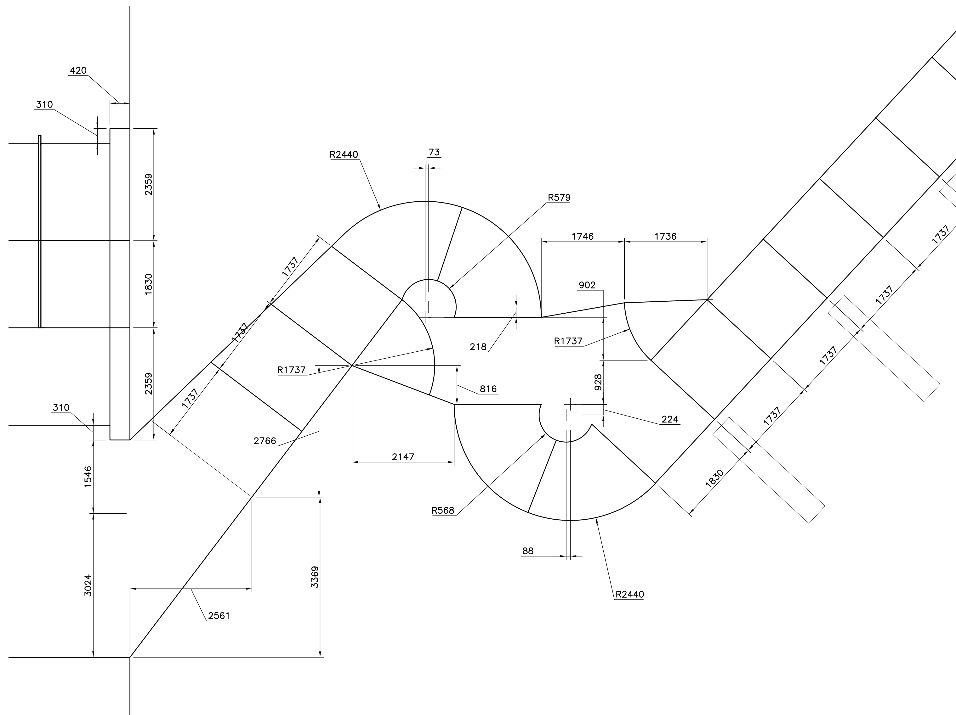
FLOW PATH DIMENSIONS
