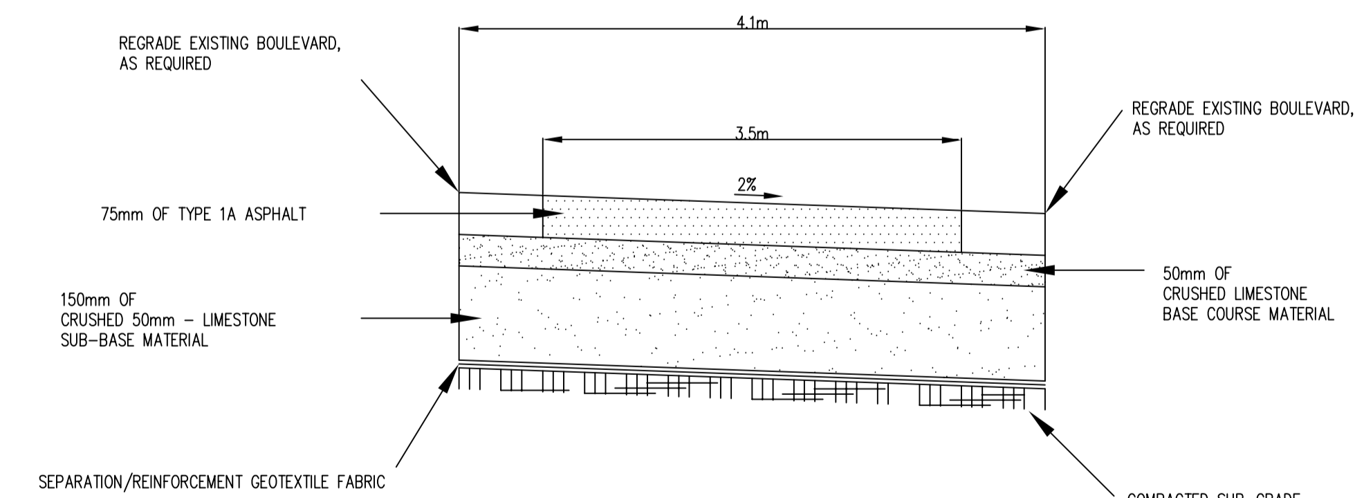
TYPICAL CROSS SECTION OF PROPOSED ASPHALT PEDESTRIAN/CYCLE PATH AT INTERSECTION TIE-IN N.T.S.
