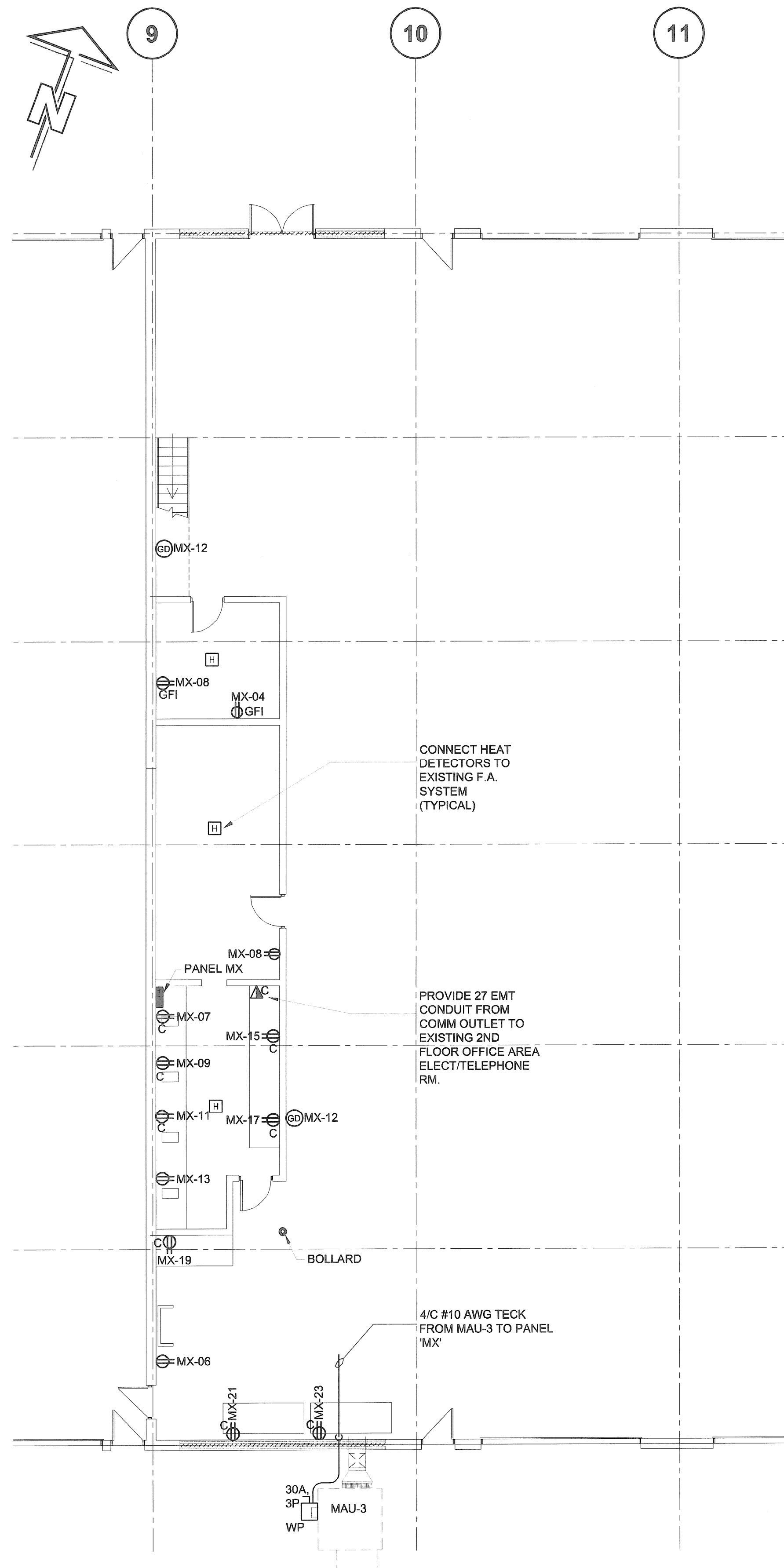
MAIN FLOOR PLAN - POWER
