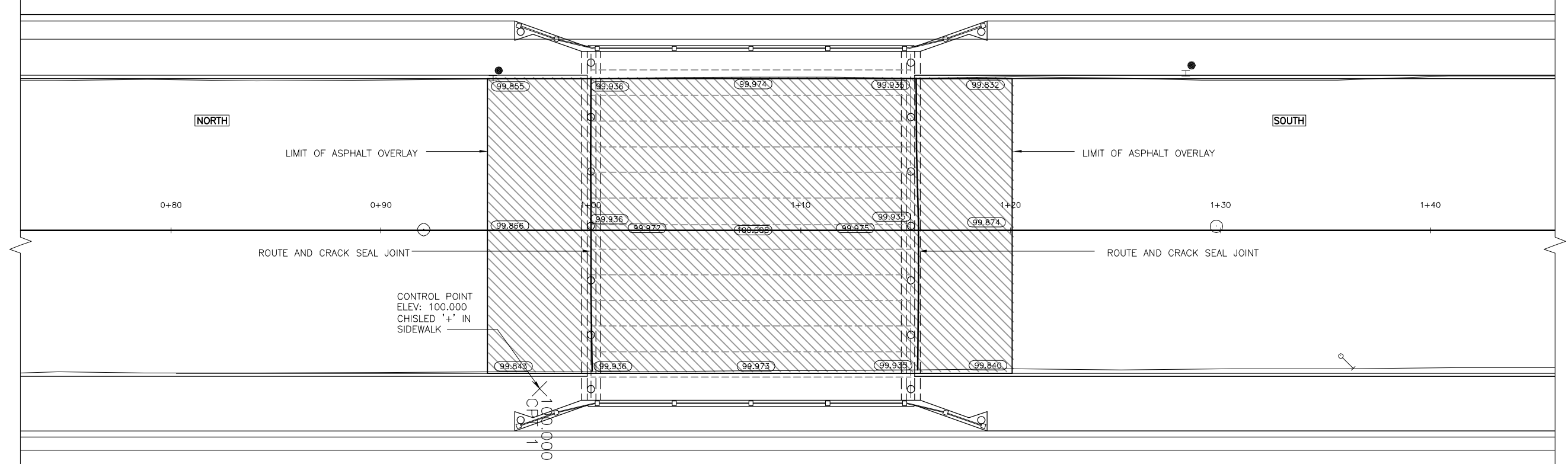
BRIDGE - PLAN SCALE: 1:100
