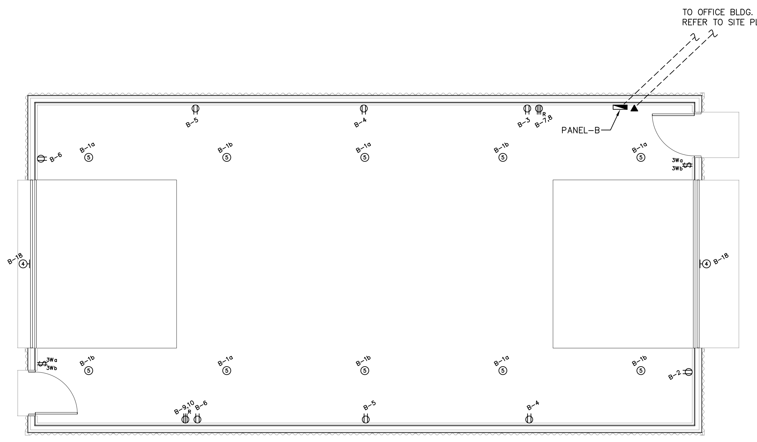
2 COLD STORAGE BUILDING ELECTRICAL PLAN E-2 SCALE: 1:50
