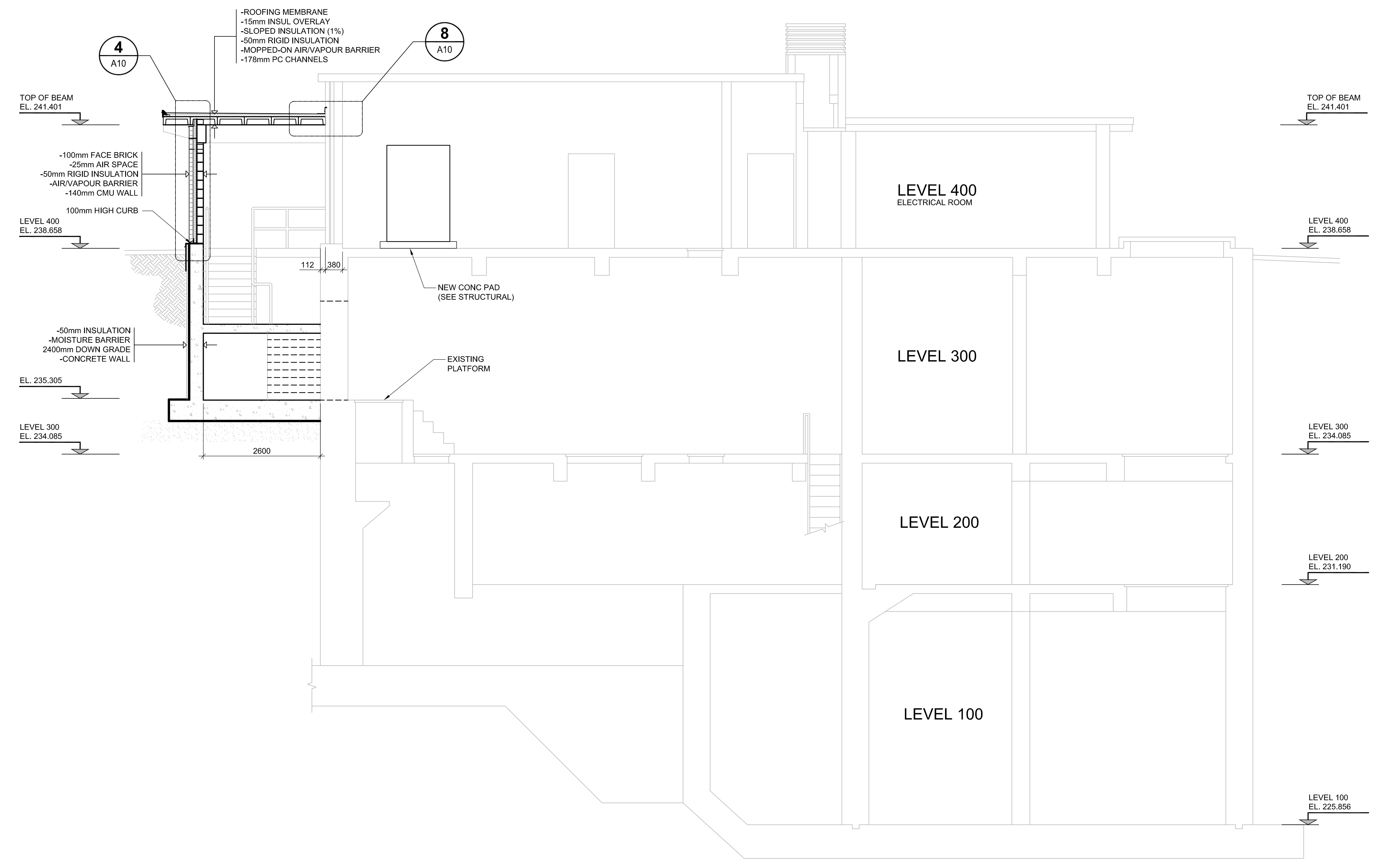
1 A05 BUILDING SECTION SCALE: 1:50
