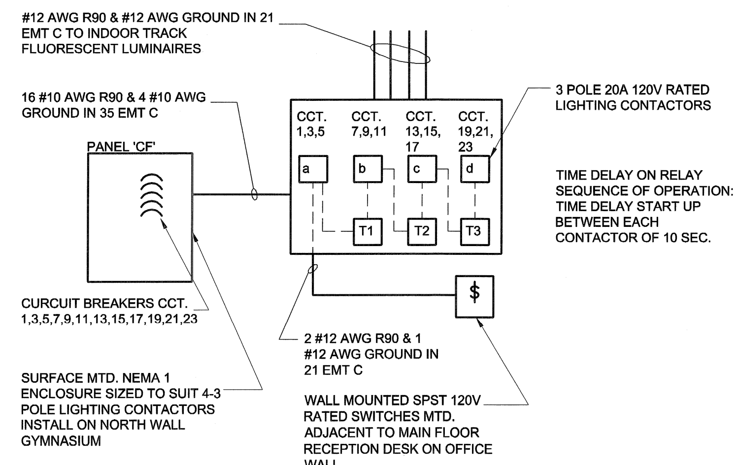
LIBRARY LIGHTING CONTROL BLOCK DIAGRAM SCALE: N.T.S.
