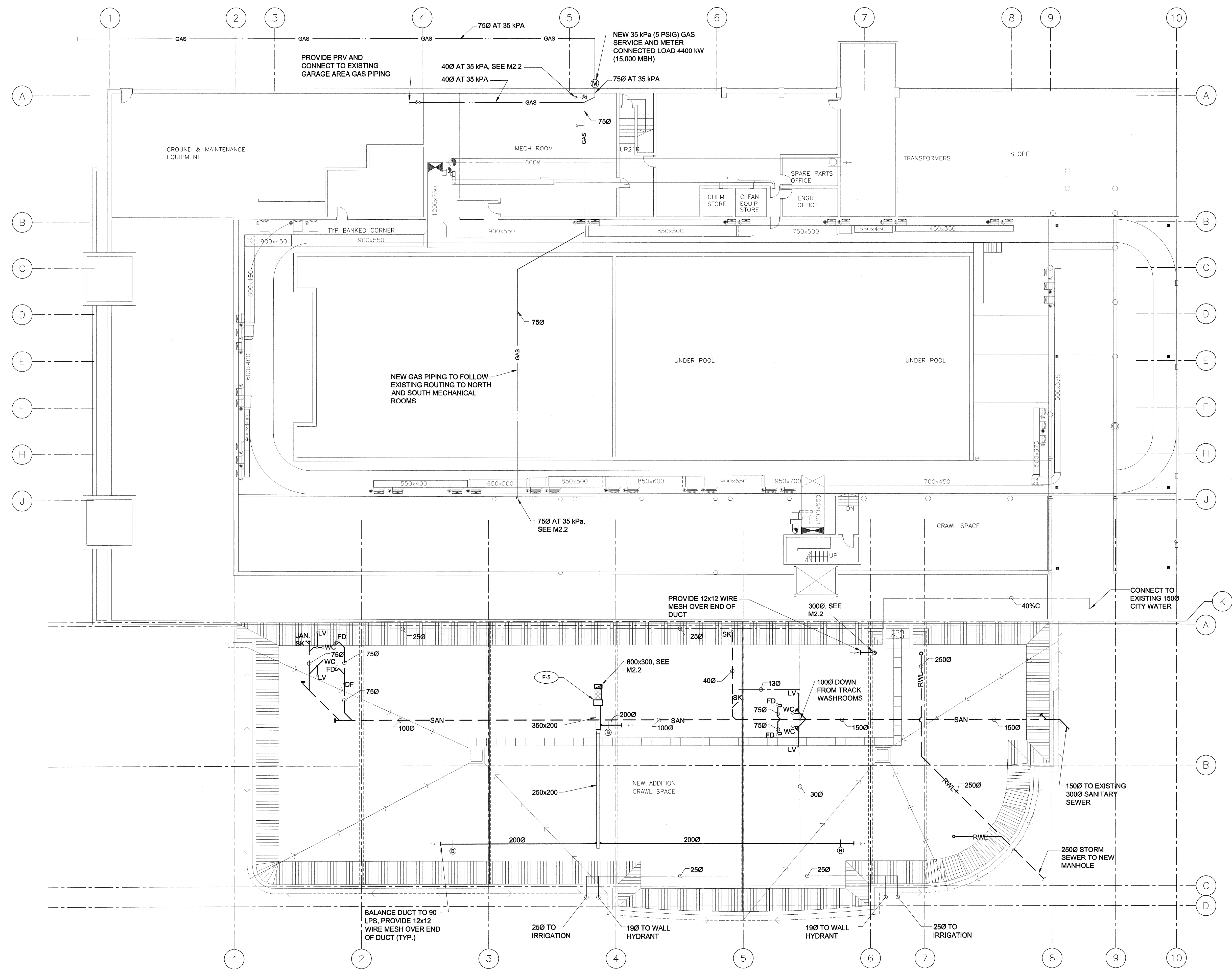
PLAN 1 M2.1 0 1500 3000 4500 mm SCALE 1:150 BASEMENT FLOOR AND CRAWL SPACE PLAN NEW CONSTRUCTION
