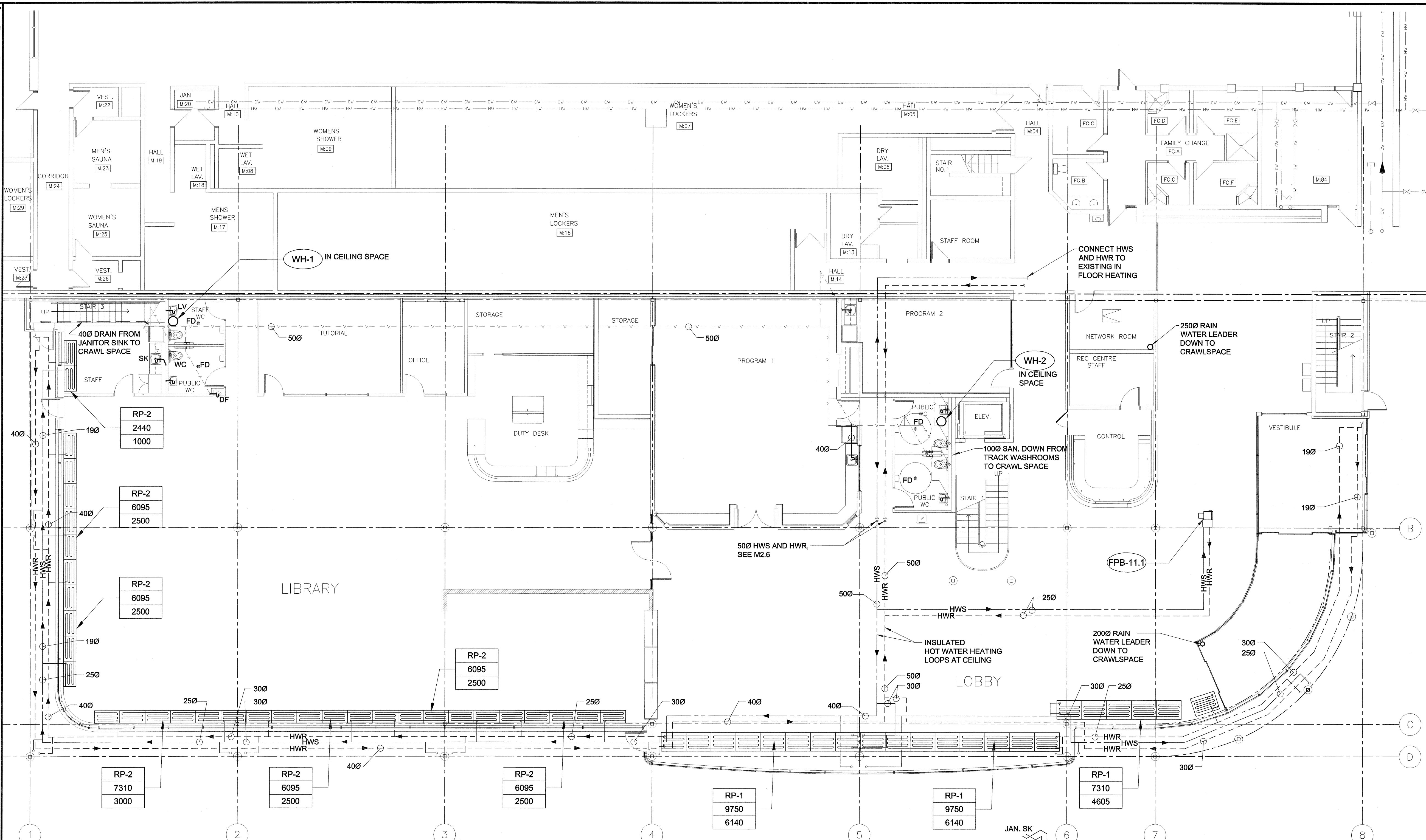
PLAN 1 SCALE 1:100 MAIN FLOOR PLUMBING NEW CONSTRUCTION
