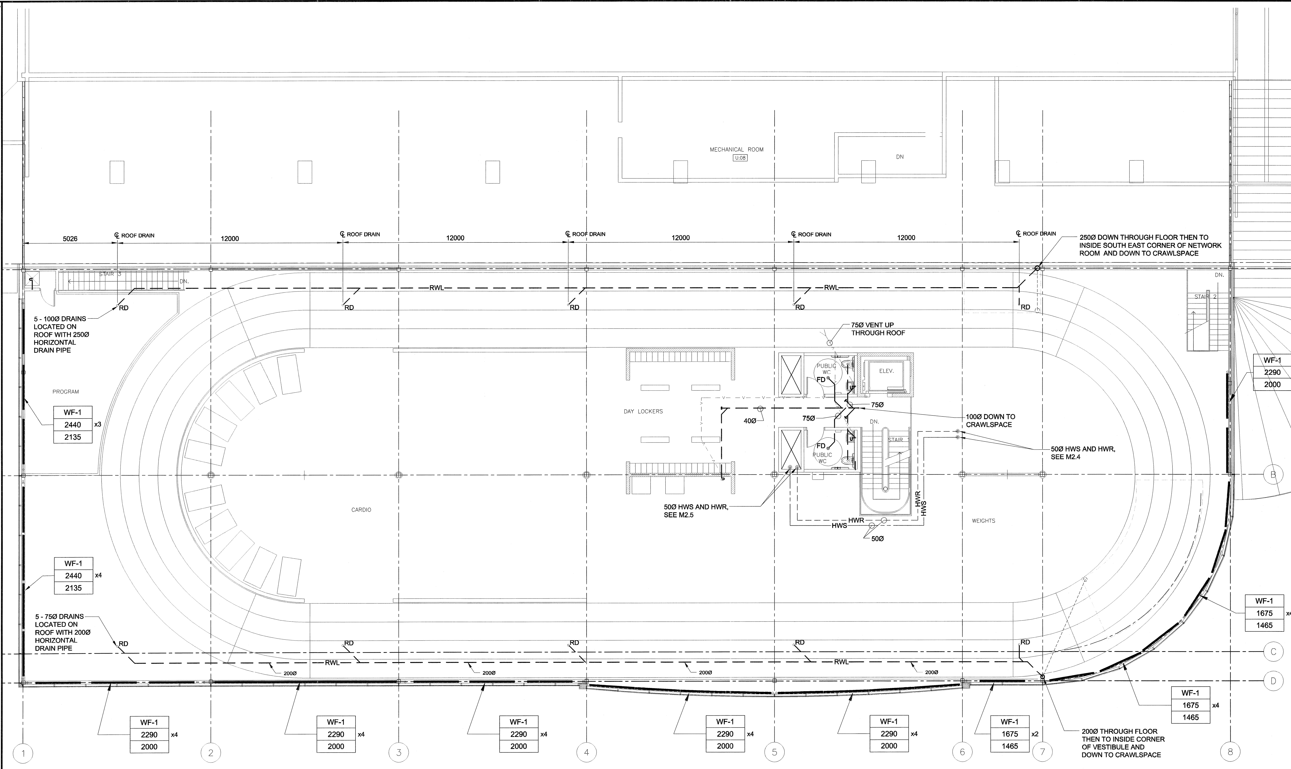
PLAN 1 M2.6 SCALE 1:100 SECOND FLOOR PLUMBING NEW CONSTRUCTION
