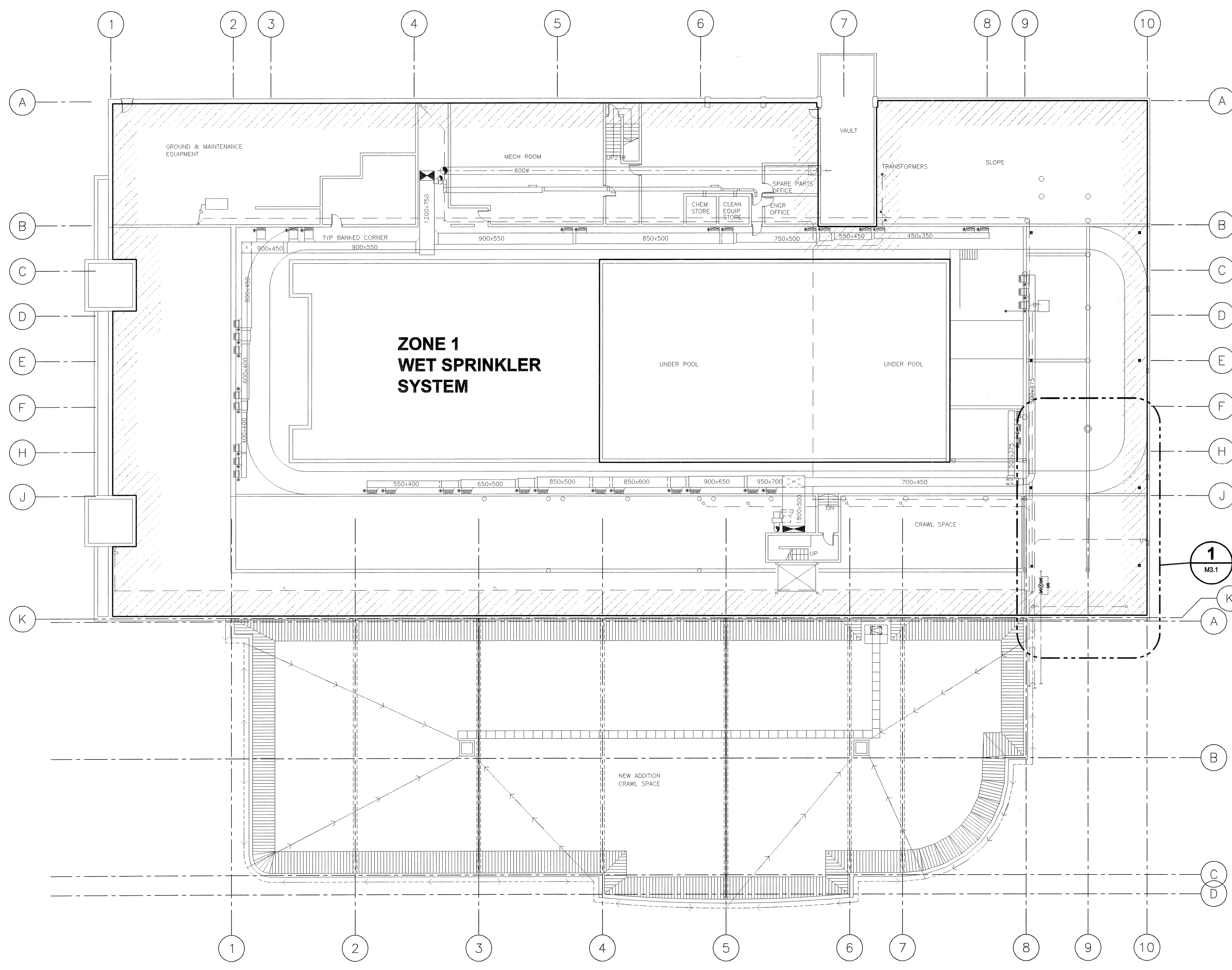
PLAN SCALE 1:200 0 2000 4000 6000 mm 1 M3.1 BASEMENT FLOOR AND CRAWL SPACE PLAN
