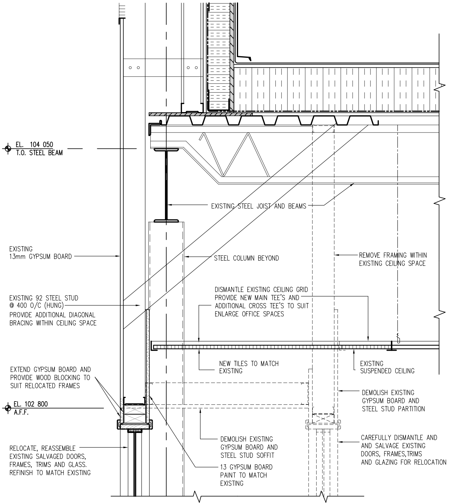
1 A.5 BULKHEAD SECTION SCALE: 1 : 10
