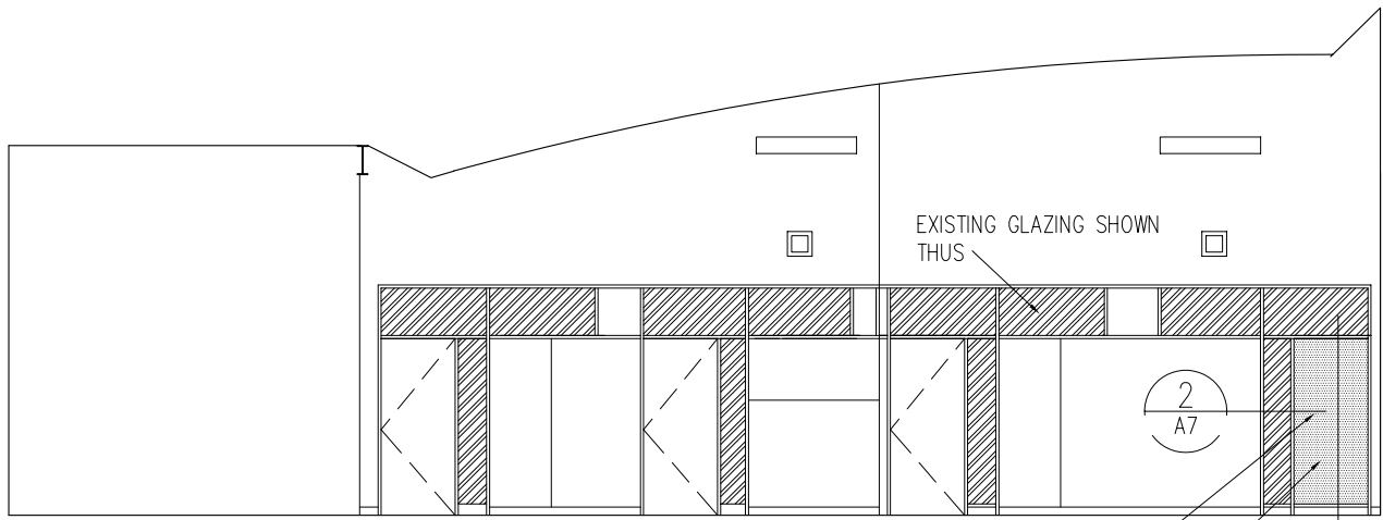
1 A.6 OPEN OFFICE AREA 1:50
