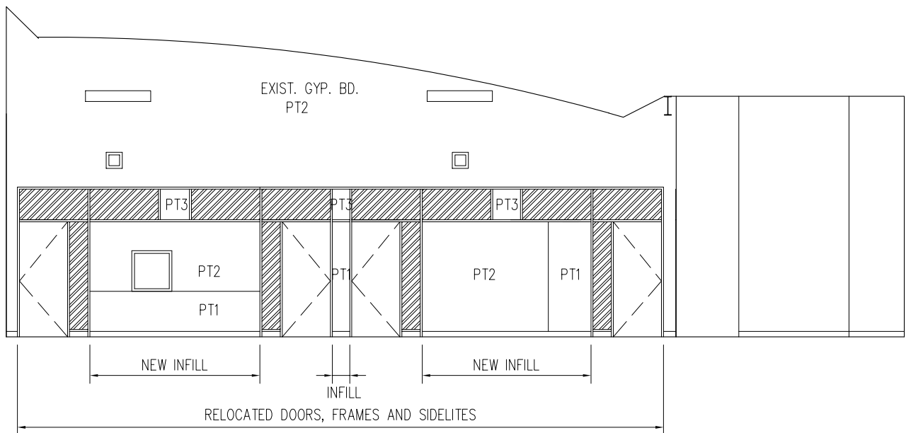
2 A.6 OPEN OFFICE AREA 1:50
