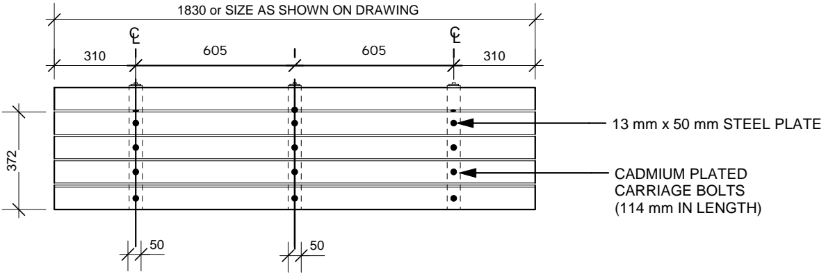
PLAN VIEW
