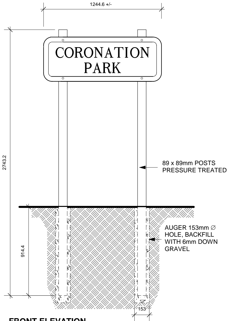
FRONT ELEVATION
