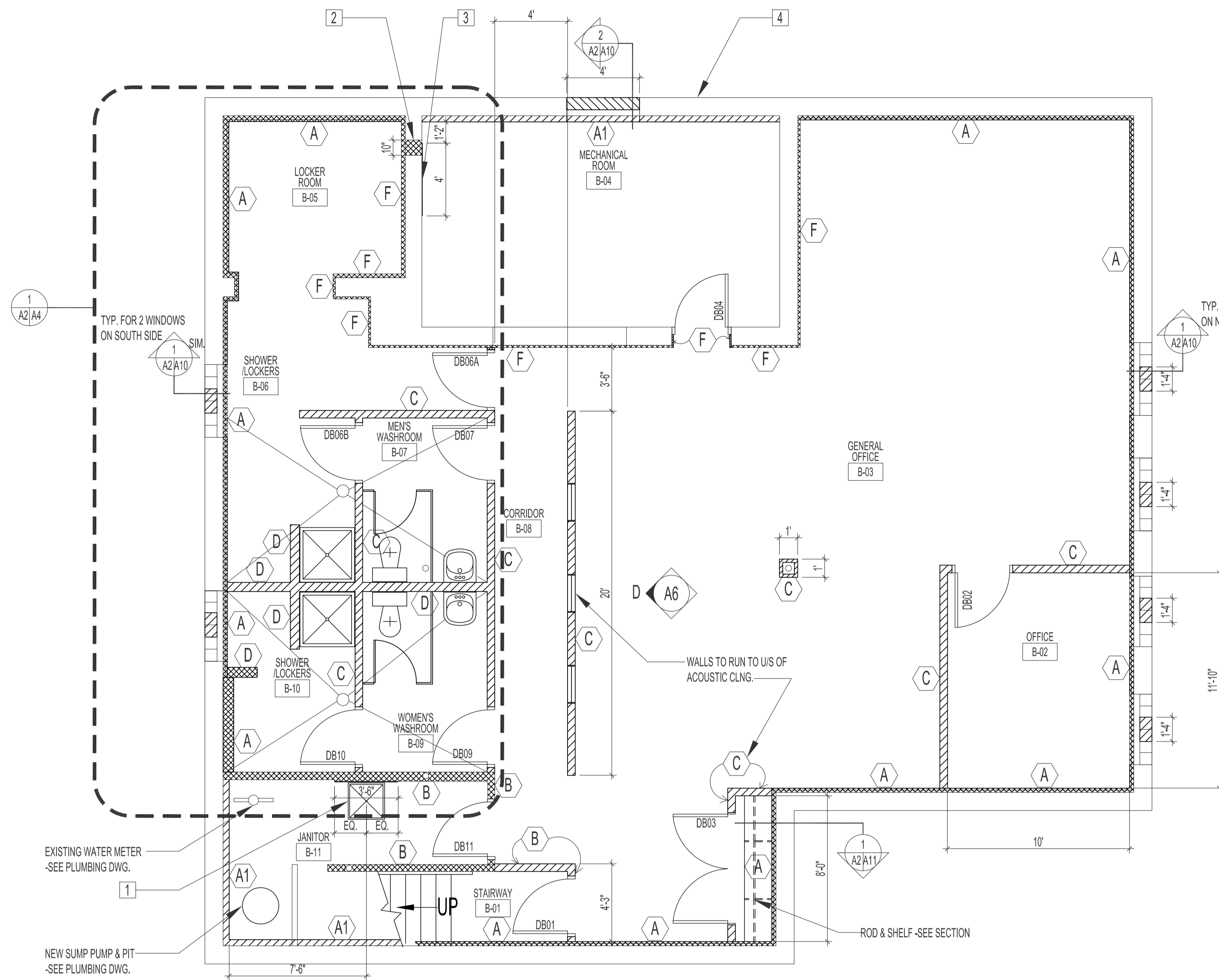
BASEMENT FLOOR PLAN - RENOVATION SCALE: 1/4"=1'-0"
