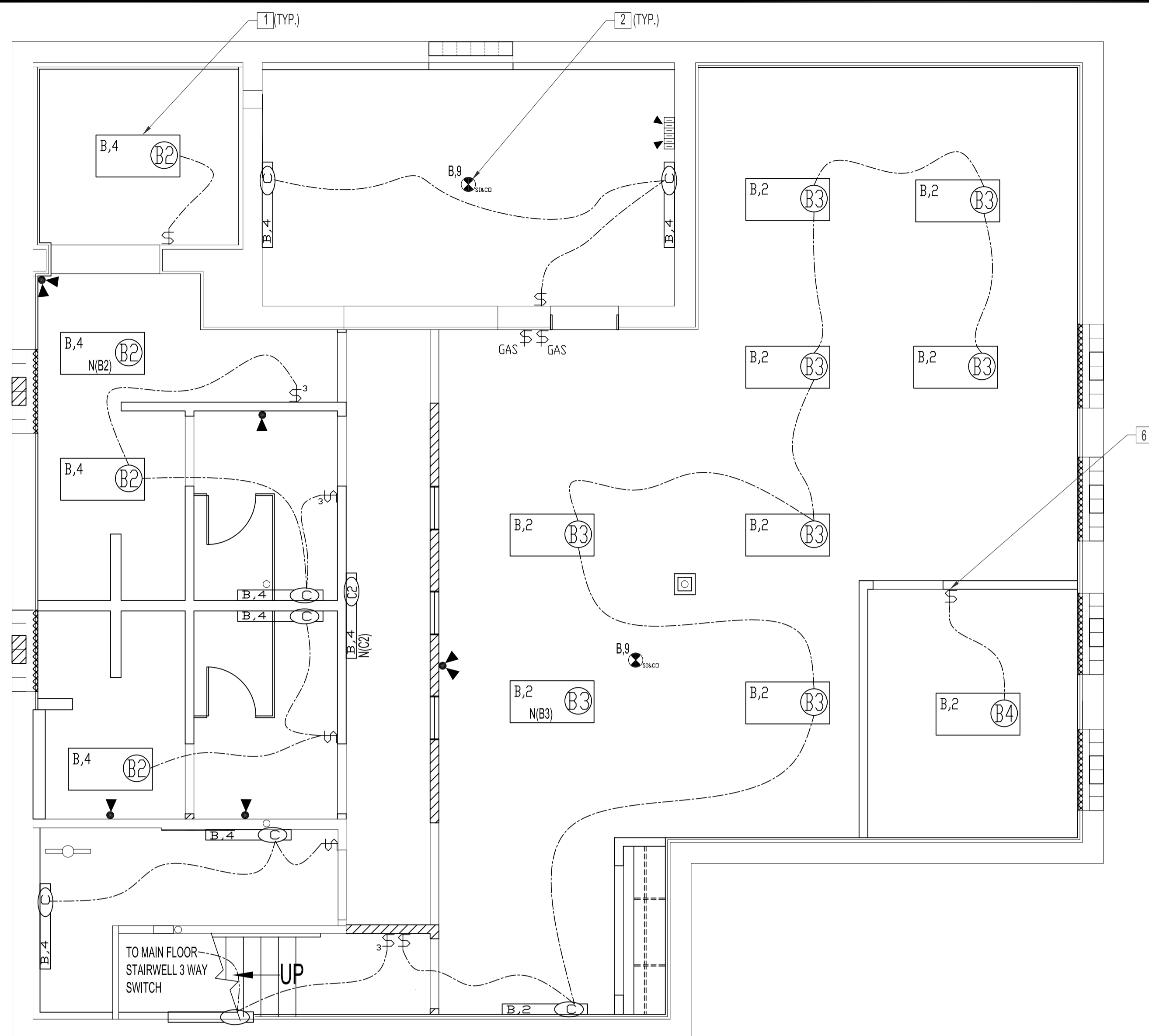
BASEMENT FLOOR PLAN - ELECTRICAL LIGHTING SCALE: 1/4"=1'-0"
