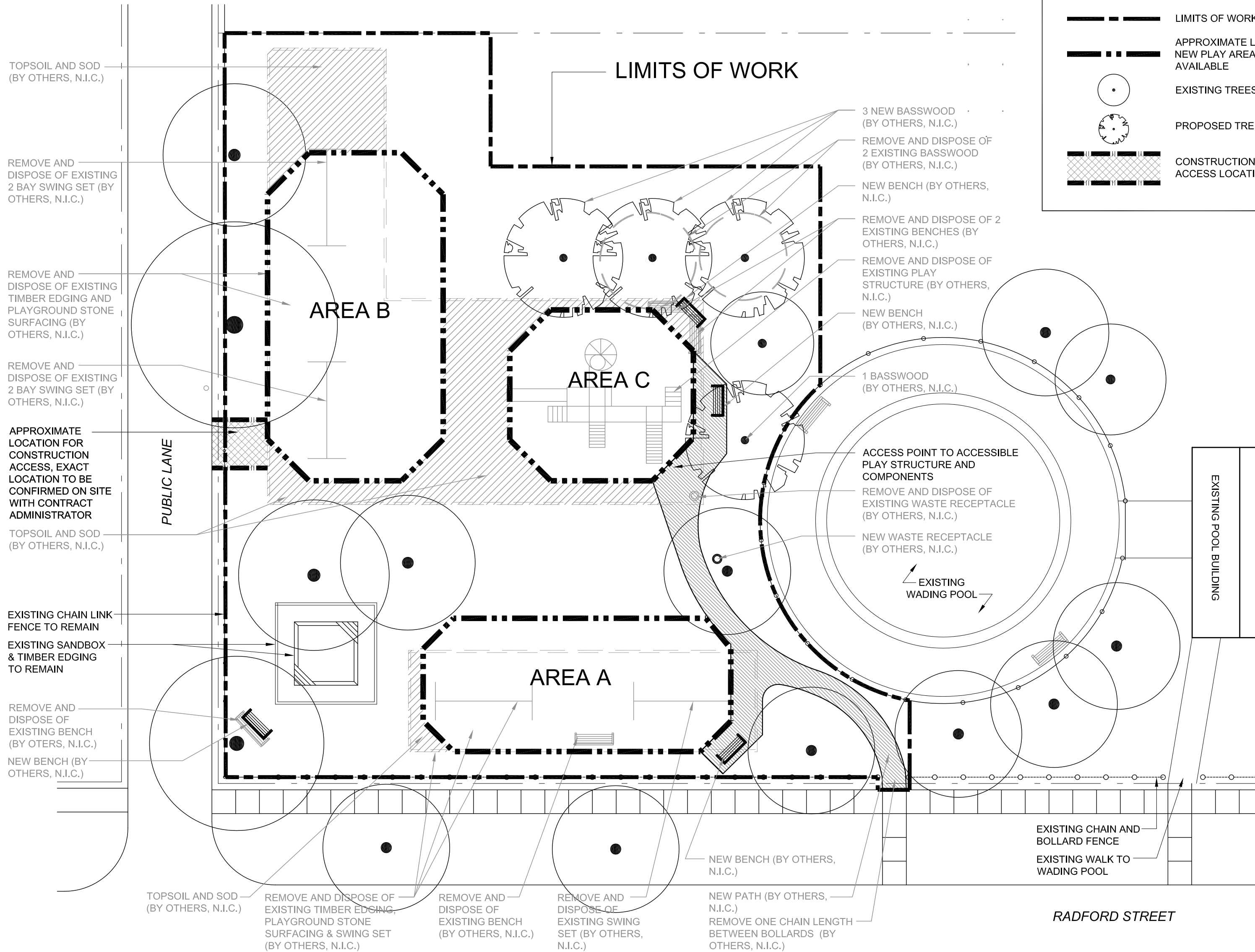
1 ROBERTSON PLAYGROUND - PROPOSED SITEPLAN RP1 SCALE 1:200
