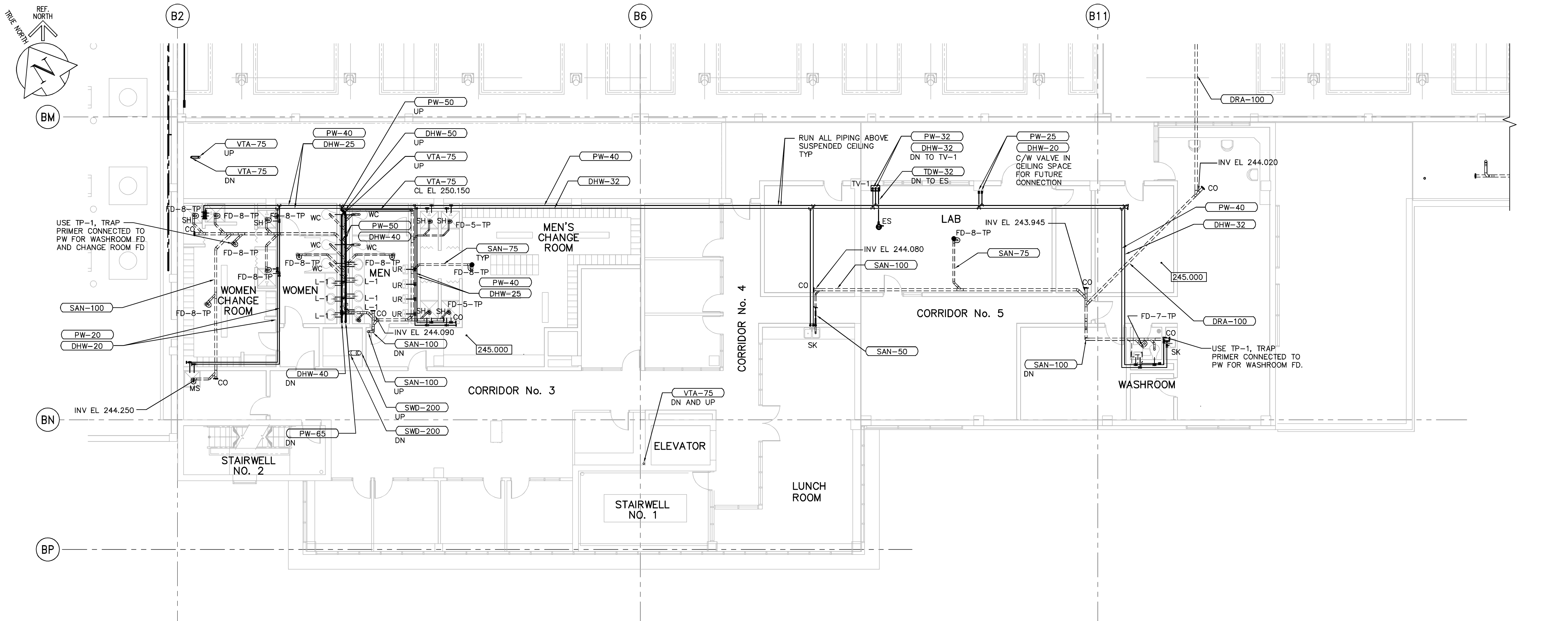
THIRD FLOOR PLAN 1:100
