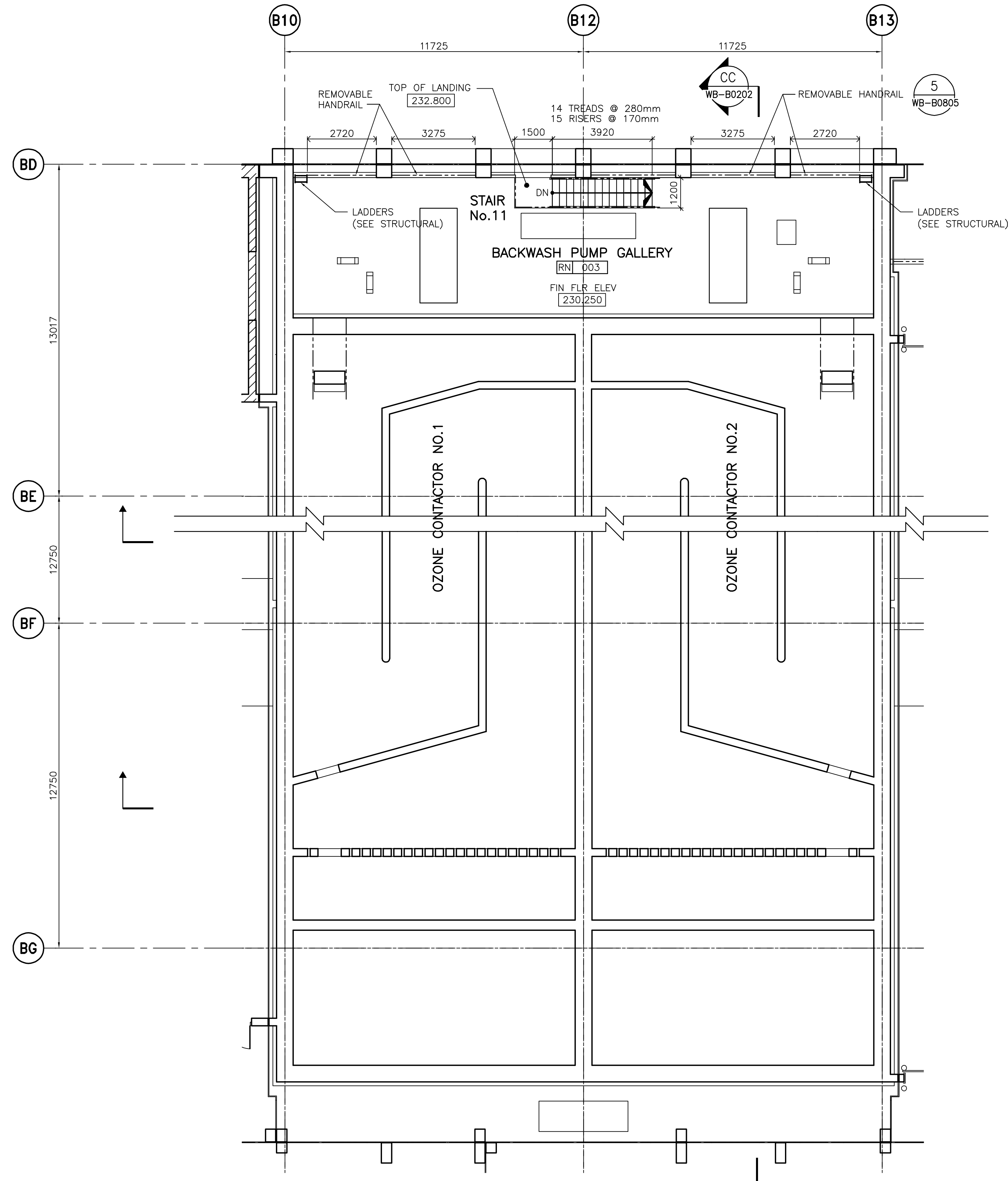
1 PARTIAL PLAN - OZONE TANK, & BACKWASH PUMP GALLERY (FIRST FLOOR) WB-B0114 1:100
