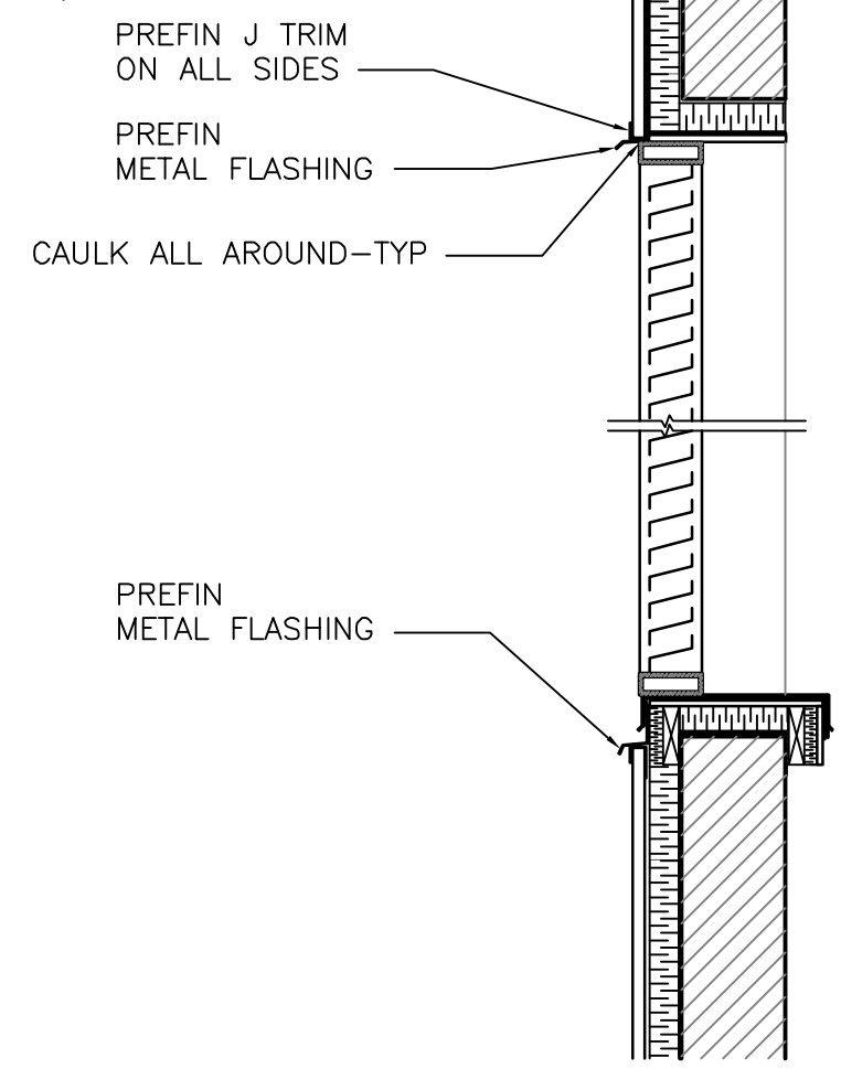
3 MECH LOUVER DETAIL @ CONC STRUCTURE WB-B0133 1:20
