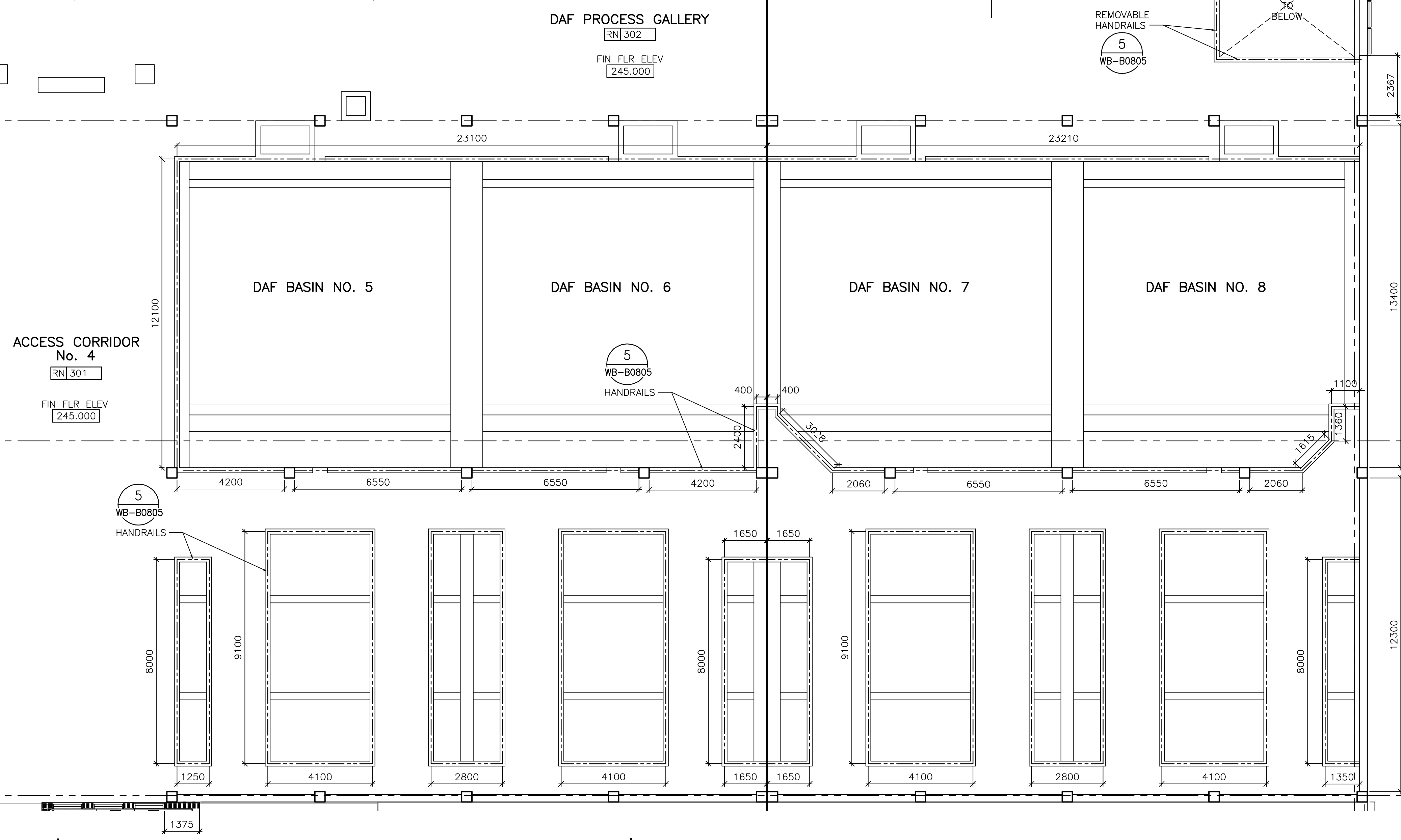
1 PARTIAL PLAN - DAF TANK & GALLERY AND PIPE GALLERY AREA (THIRD FLOOR) WB-B0137 1:100
