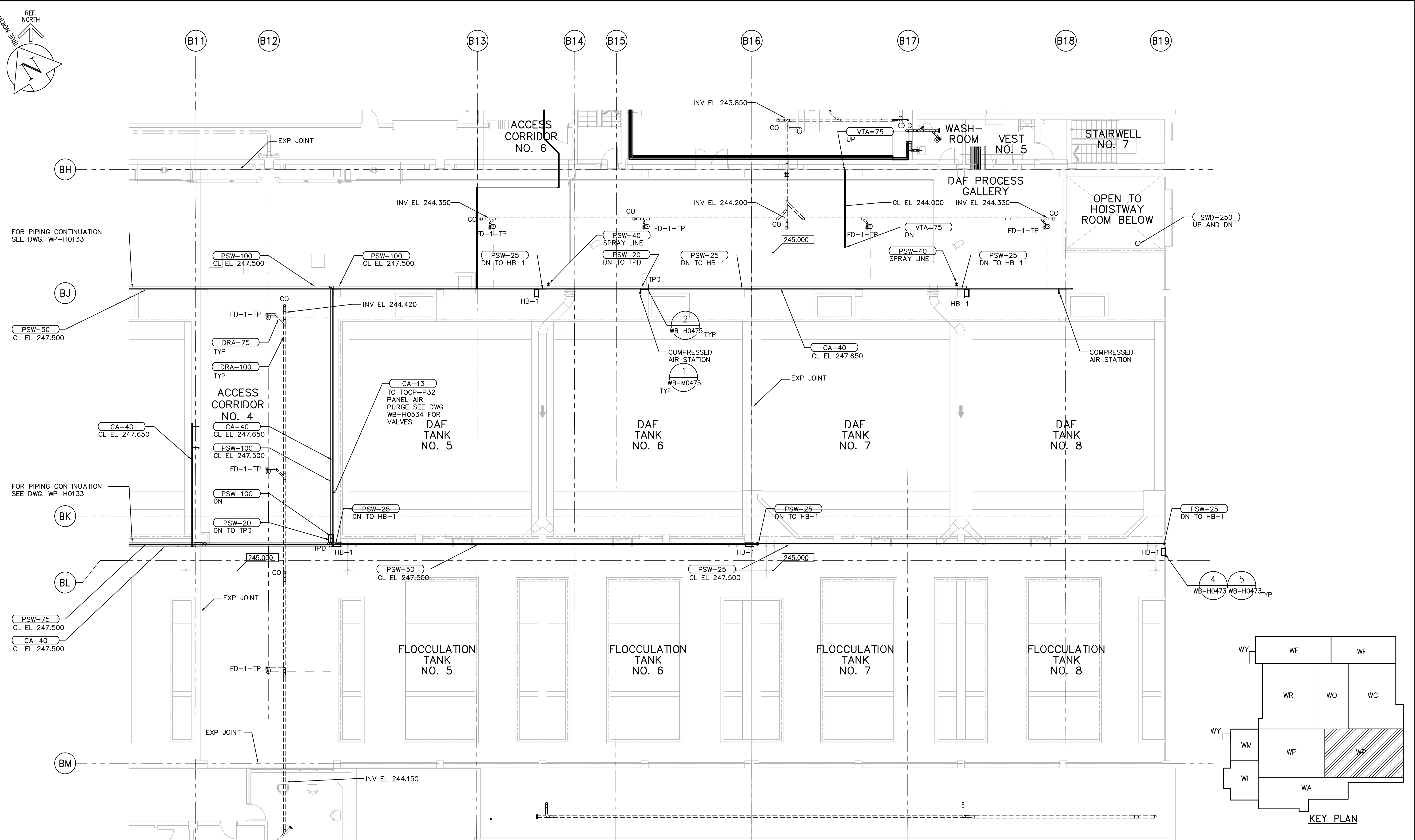
THIRD FLOOR PLAN 1:100
