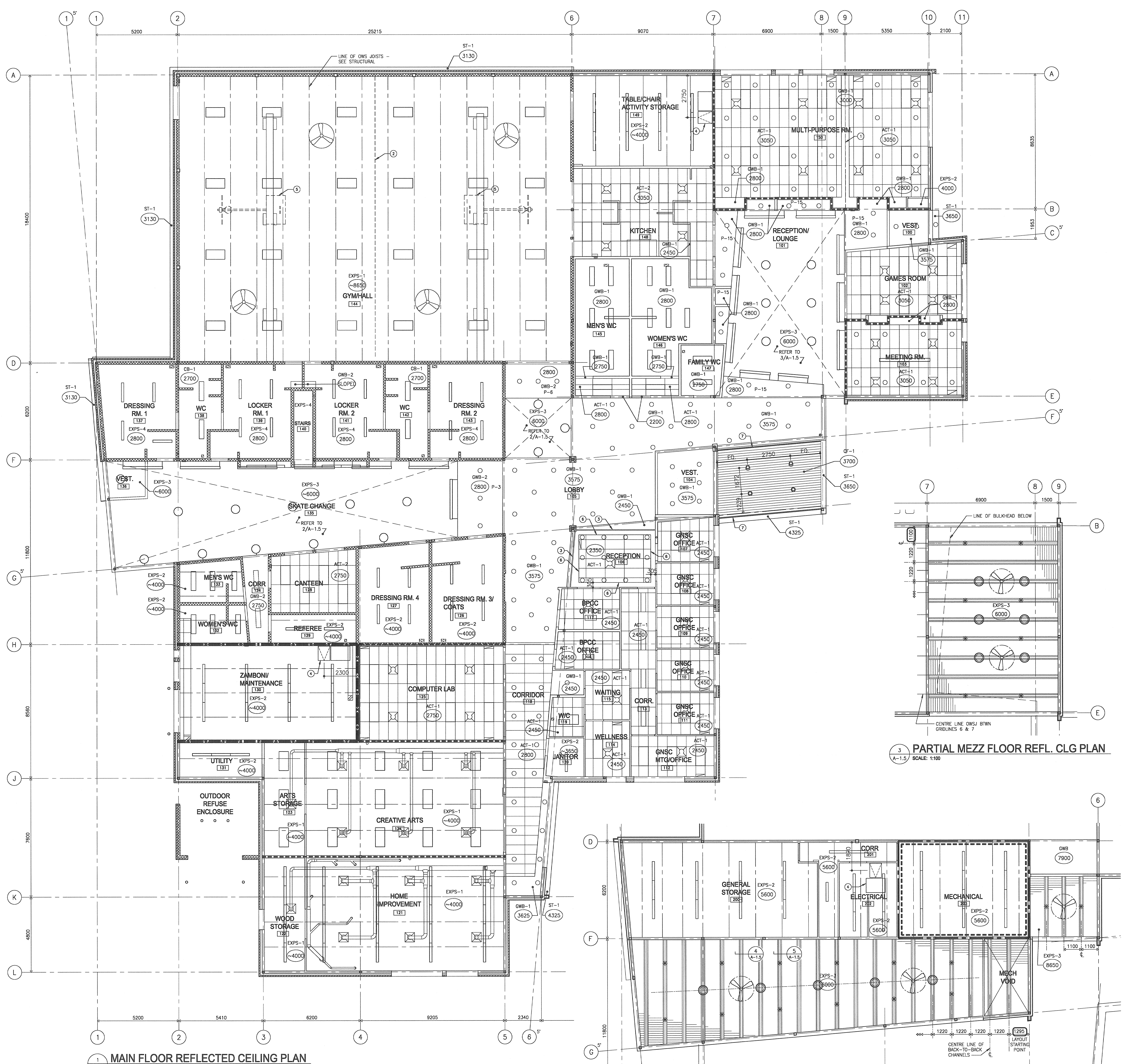
1 MAIN FLOOR REFLECTED CEILING PLAN A-1.5 SCALE: 1:100
