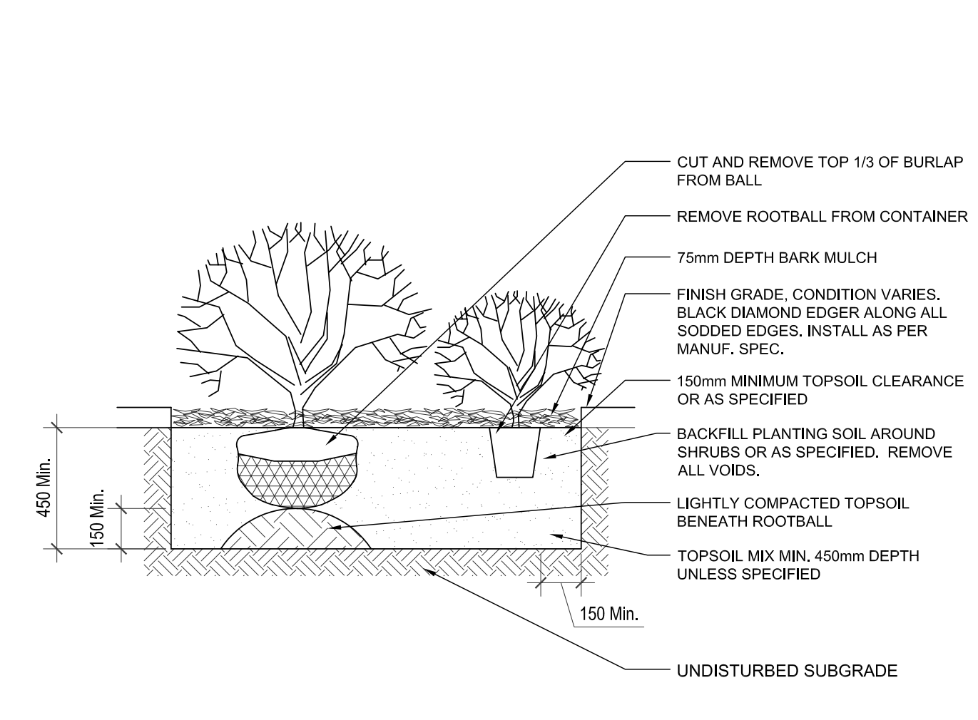
4 TYPICAL SHRUB BED DETAIL L10 SCALE 1:20
