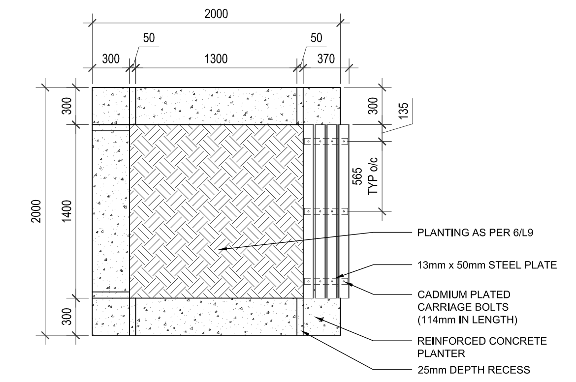
5 RAISED PLANTER WITH TREE - PLAN L10 SCALE 1:30
