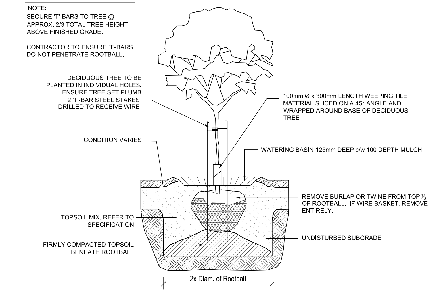
2 TYPICAL DECIDUOUS TREE PLANTING DETAIL L10 SCALE 1:30
