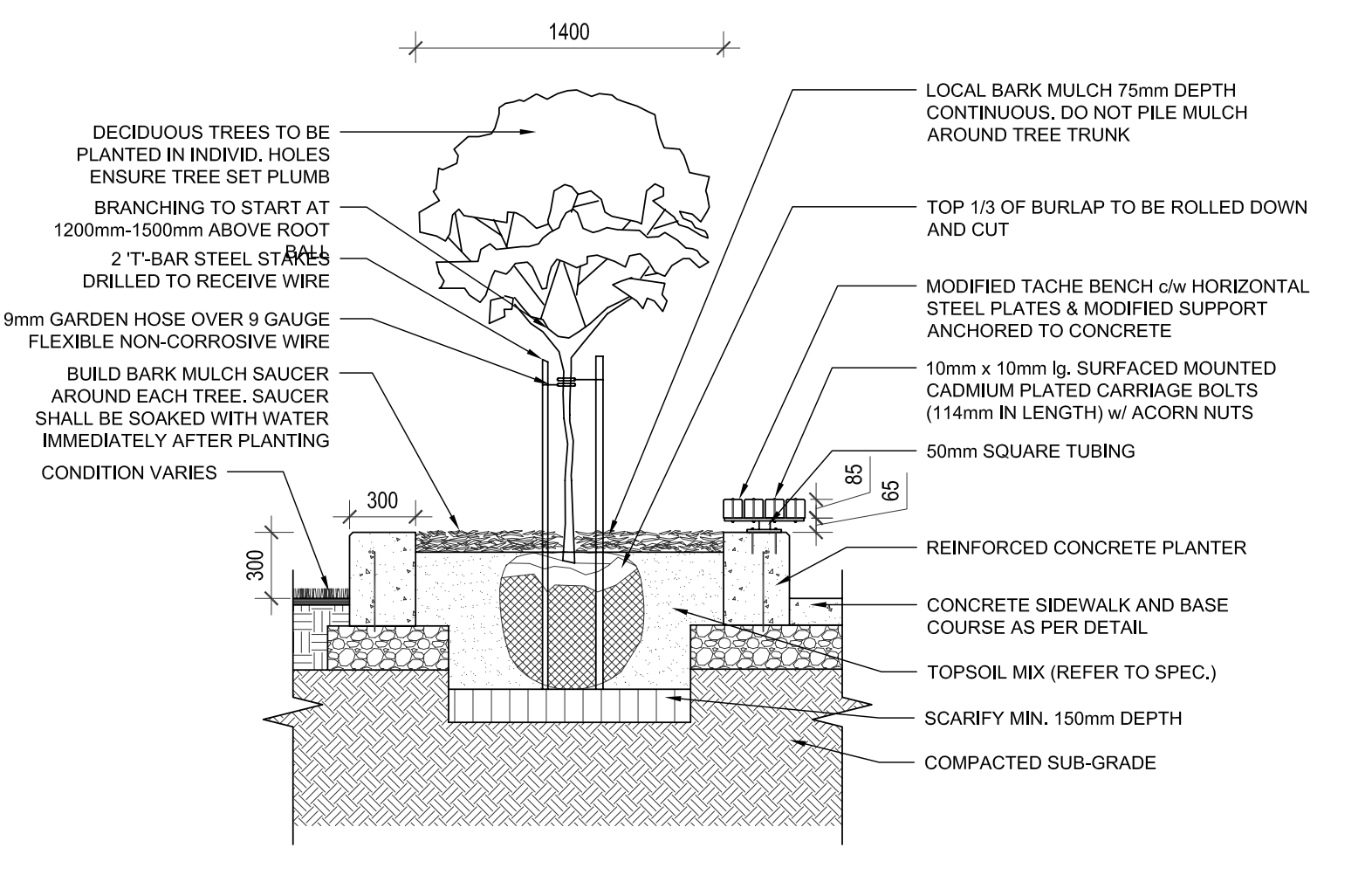
6 RAISED PLANTER WITH TREE - SECTION L10 SCALE 1:30
