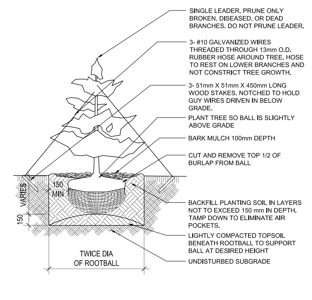
3 TYPICAL CONIFEROUS TREE PLANTING DETAIL L10 SCALE 1:30
