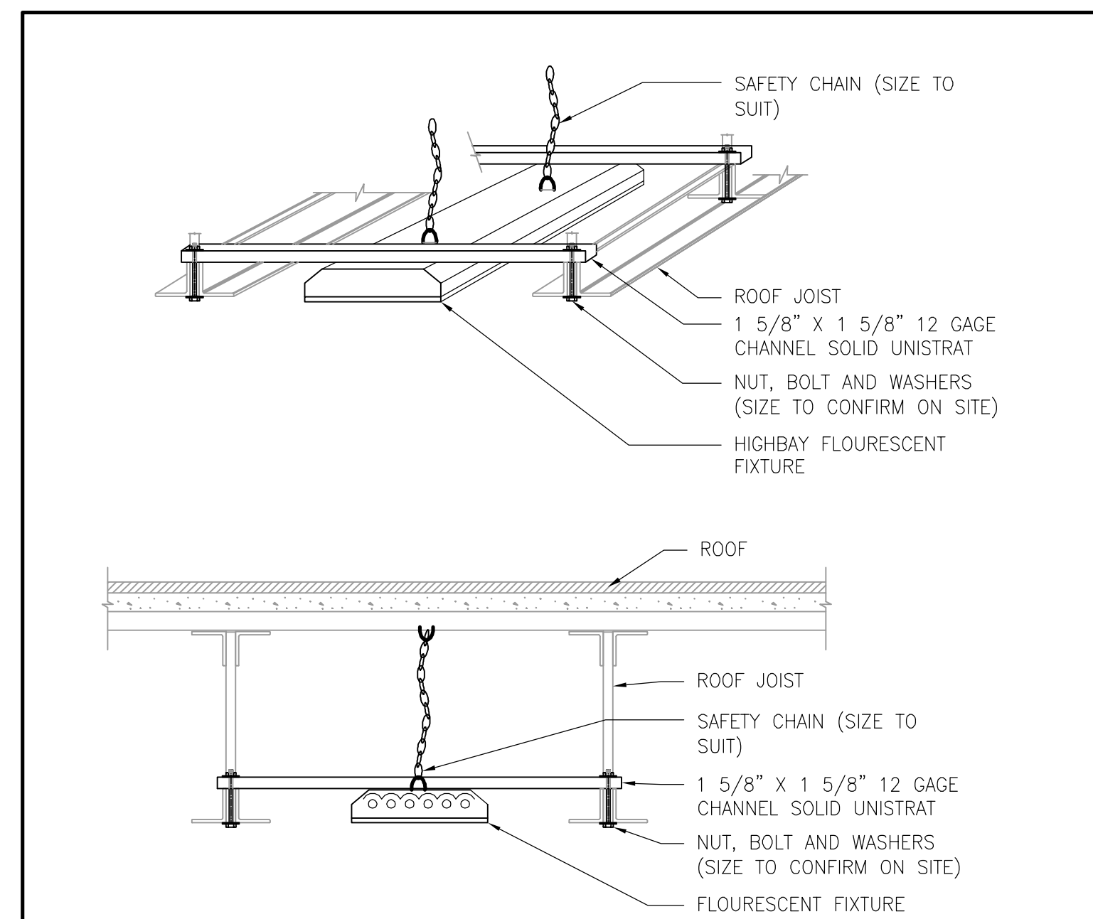
8 ACCESSIBLE CONTROL DETAIL E5.0 NTS
